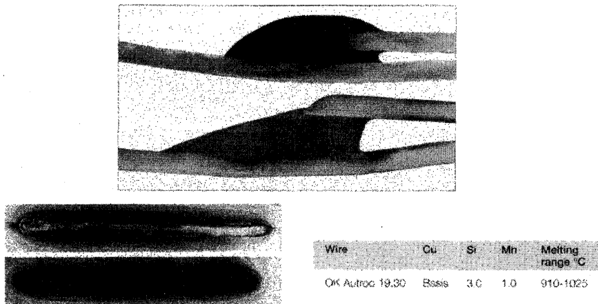
Fig.4 Samples of arc brazing.
