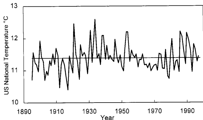
Fig. 4. Annual mean surface temperatures in the contiguous United States between 1895 and 1997, as compiled by the National Climate Data Center. 12 Horizontal line is the 103-year mean. The trend line for this 103-year period has a slope of 0.022 °C per decade or 0.22 °C per century. The trend line for 1940 to 1997 has a slope of 0.008 °C per decade or 0.08 °C per century.
