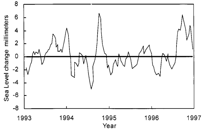
Fig. 15. Global sea level measurements from the Topex/Poseidon satellite altimeter for 1993 to 1997. 43 The instrument record gives a rate of change of minus 0.2 mm per year. 43 However, it has been reported that 50-year tide gauge measurements give plus 1.8 mm per year. A correction of plus 2.3 mm per year was added to the satellite data based on comparison to selected tide gauges to get a value of plus 2.1 mm per year or 8 inches per century. 43
