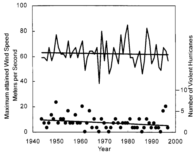
Fig. 16. Annual numbers of violent hurricanes and maximum attained wind speeds during those hurricanes in the Atlantic Ocean. 46 Slopes of the trend lines are minus 0.25 hurricanes per decade and minus 0.33 meters per second maximum attained wind speed per decade.
