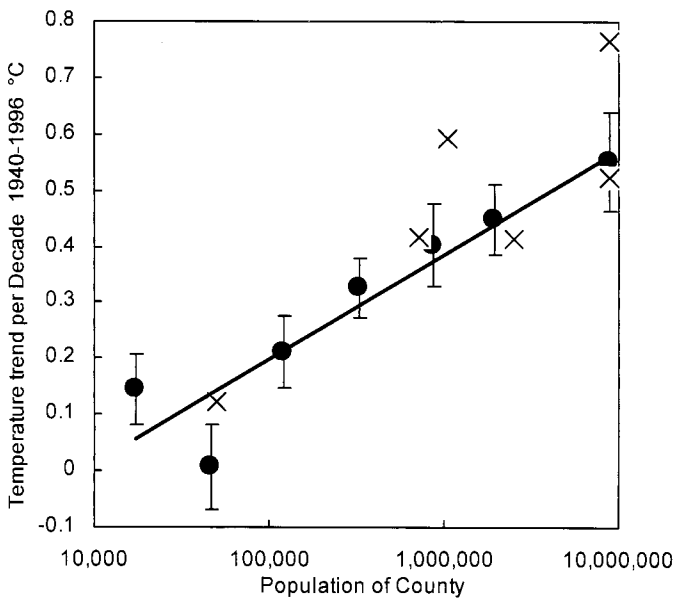
Fig. 13. Surface temperature trends for the period of 1940 to 1996 from 107 measuring stations in 49 California counties. 39,40 After averaging the means of the trends in each county, counties of similar population were combined and plotted as closed circles along with the standard errors of their means. The six measuring stations in Los Angeles County were used to calculate the standard error of that county, which is plotted alone at the county population of 8.9 million. The "urban heat island effect" on surface measurements is evident. The straight line is a least-squares fit to the closed circles. The points marked "X" are the six unadjusted station records selected by NASA GISS 23,33,34 for use in their estimate of global temperatures as shown in figure 12.
