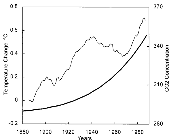
Fig. 12. Eleven-year moving average of global surface temperature, as estimated by NASA GISS 23,33,34 plotted as deviation from 1890 (left axis and light line), as compared with atmospheric CO 2 (right axis and dark line). 2 Approximately 82% of the increase in CO 2 occurred after the temperature maximum in 1940, as is shown in figure 1.
