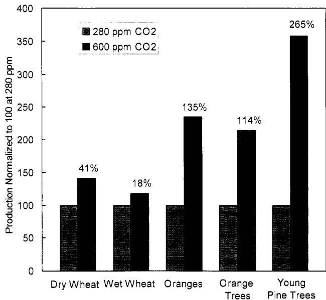
Fig. 23. Calculated growth rate enhancement of wheat, young orange and very young pine trees already taking place as a result of atmospheric enrichment by CO 2 during the past two centuries (a) and expected to take place as a result of atmospheric enrichment by CO 2 to a level of 600 ppm (b).
