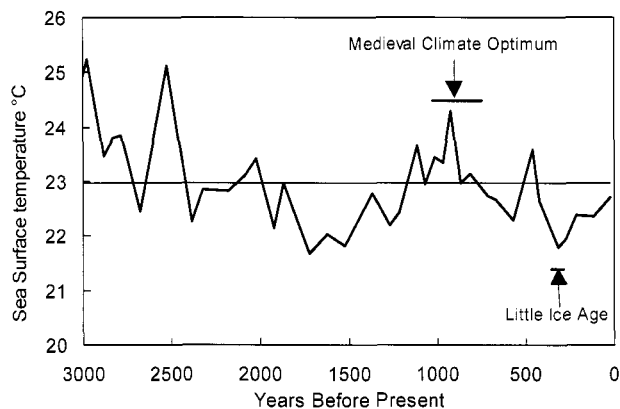
Fig. 2. Surface temperatures in the Sargasso Sea (with time resolution of about 50 years) ending in 1975 as determined by isotope ratios of marine organism remains in sediment at the bottom of the sea. 7 The horizontal line is the average temperature for this 3,000 year period. The Little Ice Age and Medieval Climate Optimum were naturally occurring, extended intervals of climate departures from the mean.
