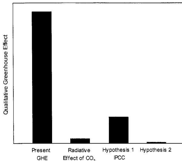
Fig. 9. Qualitative illustration of greenhouse warming. Present: the current greenhouse effect from all atmospheric phenomena. Radiative effect of CO 2 : added greenhouse radiative effect from doubling CO 2 without consideration of other atmospheric components. Hypothesis 1 IPCC: hypothetical amplification effect assumed by IPCC. Hypothesis 2: hypothetical moderation effect.
