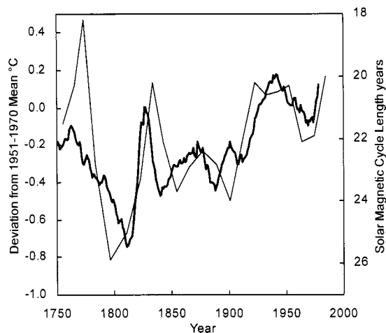
Fig. 3. Moving 11-year average of terrestrial Northern Hemisphere temperatures as deviations in °C from the 1951-1970 mean — left axis and darker line. 8,9 Solar magnetic cycle lengths — right axis and lighter line. 10 The shorter the magnetic cycle length, the more active, and hence brighter, the sun.
