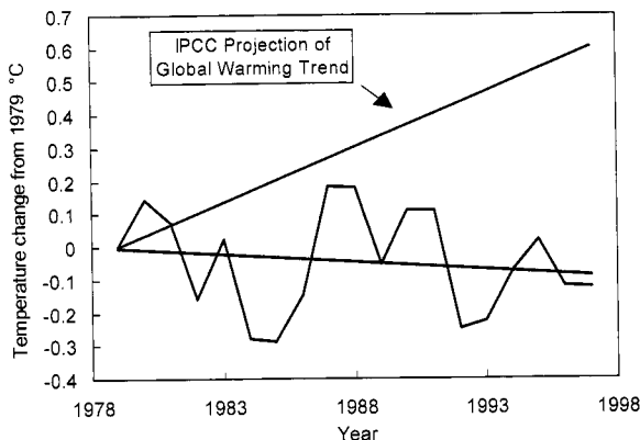
Fig. 11. Global annual lower tropospheric temperatures as measured by satellite MSU between latitudes 83 N and 83 S 17,18 plotted as deviations from the 1979 value. The trend line of these experimental measurements is compared with the corresponding trend line predicted by the International Panel on Climate Change (IPCC) computer climate models. 14
