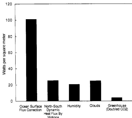
Fig. 10. The radiative greenhouse effect of doubling the concentration of atmospheric CO 2 (right bar) as compared with four of the uncertainties in the computer climate models. 14,28
