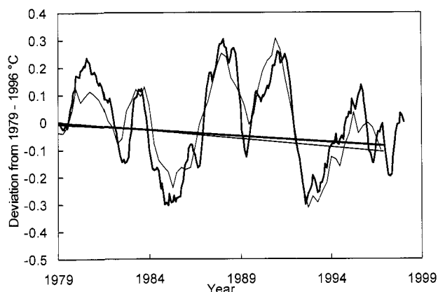
Fig. 7. Global radiosonde balloon temperature (light line) 15 and global satellite MSU temperature (dark line) 17,18 from figures 5 and 6 plotted with 6-month smoothing. Both sets of data are graphed as deviations from their respective means for 1979 to 1996. The 1979 to 1996 slopes of the trend lines are minus 0.060 °C per decade for balloon and minus 0.045 for satellite.
