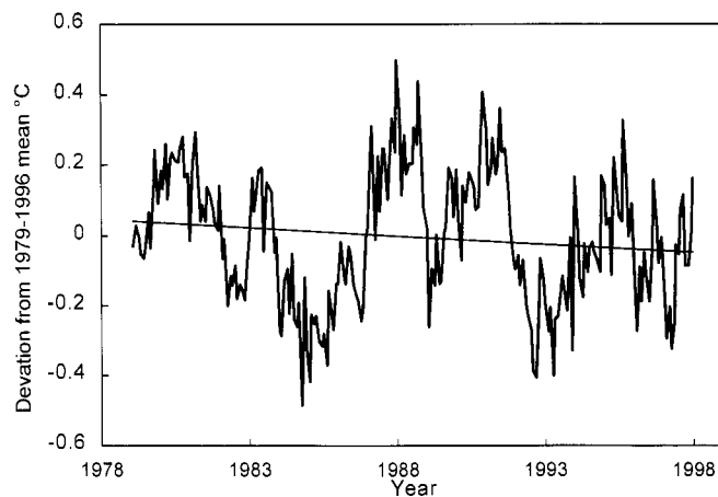
Fig. 6. Satellite Microwave Sounding Unit, MSU, measurements of global lower tropospheric temperatures between latitudes 83 N and 83 S from 1979 to 1997. 17,18 Temperatures are monthly averages and are graphed as deviations from the mean temperature for 1979 to 1996. Linear trend line for 1979 to 1997 is shown. The slope of this line is minus 0.047 °C per decade. This record of measurements began in 1979.
