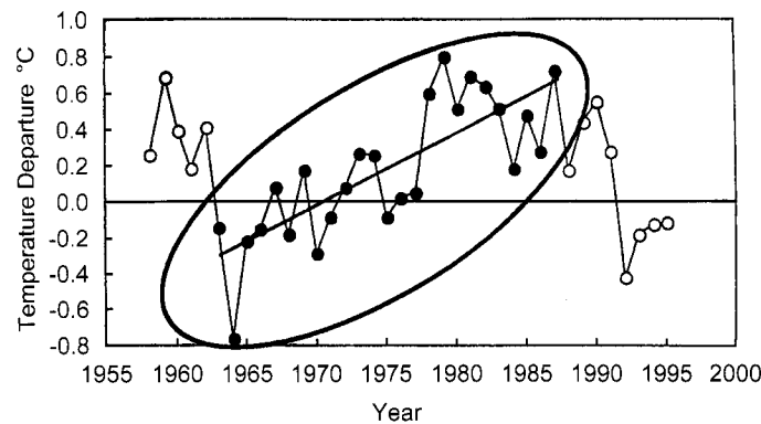
Fig. 14. The solid circles in the oval are tropospheric temperatures for the Southern Hemisphere between latitudes 30 S and 60 S, published in 1996 41 in support of computer-model-projected warming. Later in 1996, the study was refuted by a longer set of data, as shown by the open circles. 42
