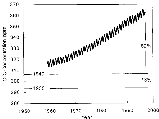
Fig. 1. Atmospheric CO 2 concentrations in parts per million by volume, ppm, at Mauna Loa, Hawaii. These measurements agree well with those at other locations. 1 Periodic cycle is caused by seasonal variations in CO 2 absorption by plants. Approximate global level of atmospheric CO 2 in 1900 and 1940 is also displayed. 2
