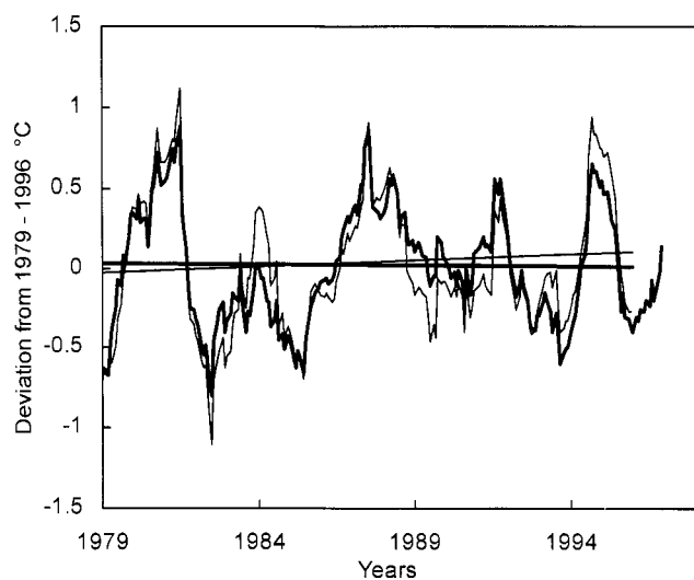
Fig. 8. Tropospheric temperature measurements by satellite MSU for North America between 30° to 70° N and 75° to 125° W (dark line) 17,18 compared with the surface record for this same region (light line), 24 both plotted with 12-month smoothing and graphed as deviations from their means for 1979 to 1996. The slope of the satellite MSU trend line is minus 0.01 °C per decade, while that for the surface trend line is plus 0.07 °C per decade. The correlation coefficient for the unsmoothed monthly data in the two sets is 0.92.
