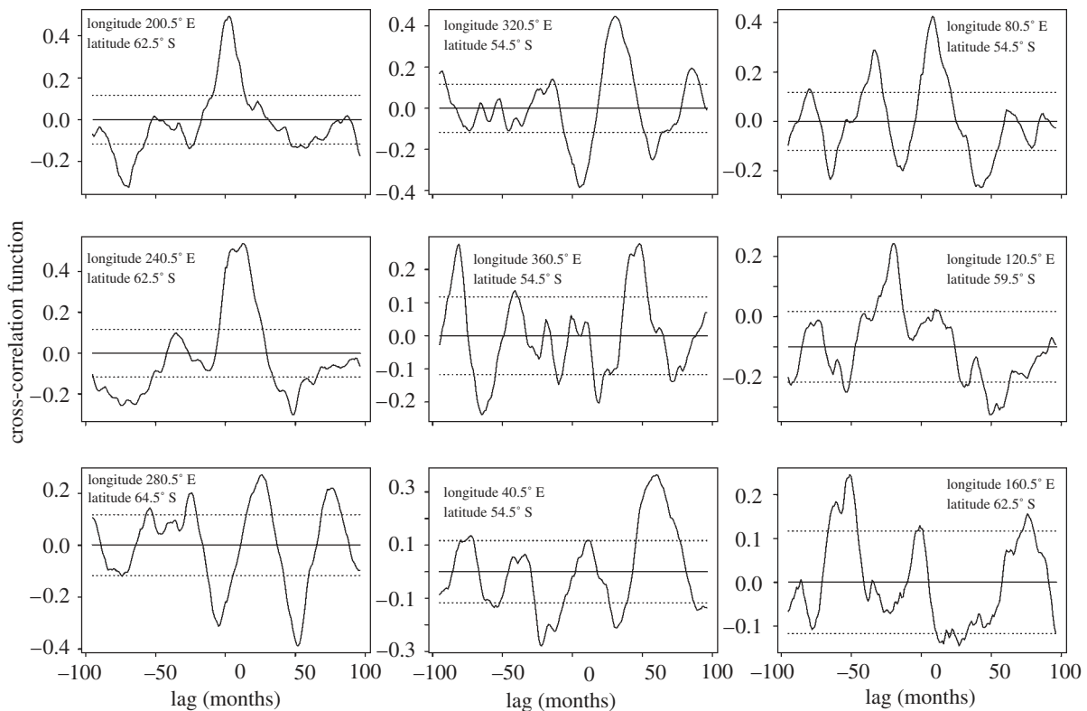
Figure 2. Plots of the cross-correlation function between the El Niño 4 region ( 5^{\circ} N to 5^{\circ} S, 160^{\circ} E to 50^{\circ} W; http://www.cpc.noaa.gov/data/indices/sstoi.indices ) and sea surface temperatures (Reynolds et al. 2002) close to the Antarctic Polar Front at longitudes 40^{\circ} , 80^{\circ} , 120^{\circ} , 160^{\circ} , 200^{\circ} , 240^{\circ} , 280^{\circ} , 320^{\circ} and 360^{\circ} E. The time-series at each longitude represents the mean temperature value from a box measuring 2^{\circ} of latitude \times 2^{\circ} of longitude. The 95% confidence limits ( \pm 1.96/\sqrt{n} where n=280 ) are shown to help indicate whether cross-correlations are significantly different from zero.
