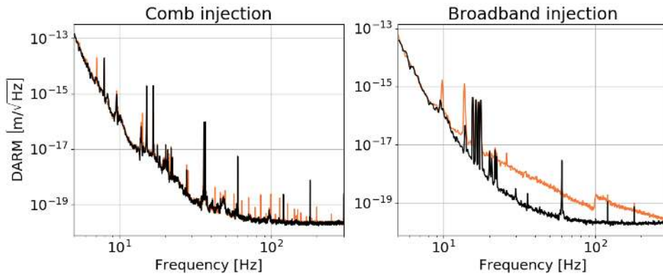
Figure 9. DARM response to old (left, comb) and new (right, broadband) magnetic injections. Black and orange lines show the DARM ASD before and during the injections, respectively. The comb injection curve is a composite of multiple comb injections, with fundamental frequencies of 7.1 Hz, 14.2 Hz, and 49.7 Hz, made at different times. The broadband injection spectrum is a composite of a 10-100 Hz injection and a 100-1000 Hz injection made at different times, hence the break at 100 Hz.
