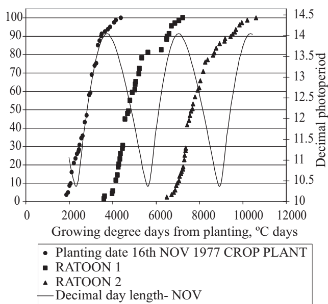
Figure 4. The cumulative (%) bunch initiation of three crop cycles of cv. 'Williams' banana planted in November 1977 at Alstonville, NSW (Lat 29°S). Curves are plotted against growing-degree-days (GDD) from planting date. The oscillating line is the photoperiod (decimal hours) and the horizontal line describes the 12 h photoperiod. Data from Turner and Hunt (1987).
