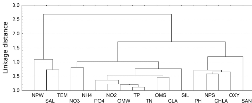
Figure 3. Cluster analysis of water column and sediment parameters. SAL, salinity; TEM, temperature; PO4, phosphate; NO2, nitrite; OMW, organic matter in water; OMS, organic matter in sediment; TP, total phosphate; TN, total nitrogen; CLA, clay; NO2, nitrate; NH4, ammonium; SIL, silt; PH, pH; OXY, dissolved oxygen; SAN, sand; CHLA, Chl- a ; NPW, N:P ratio in water; NPS, N:P ratio in sediment / Análisis de clúster de los parámetros de la columna de agua y sedimento
