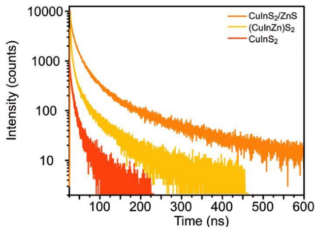
Fig. 8 Time resolved photoluminescence decay curves for the CuInS 2 core nanocrystals only, the (CuInZn) 2 S 2 quaternary alloy and the CuInS 2 /ZnS core/shell nanocrystals.
