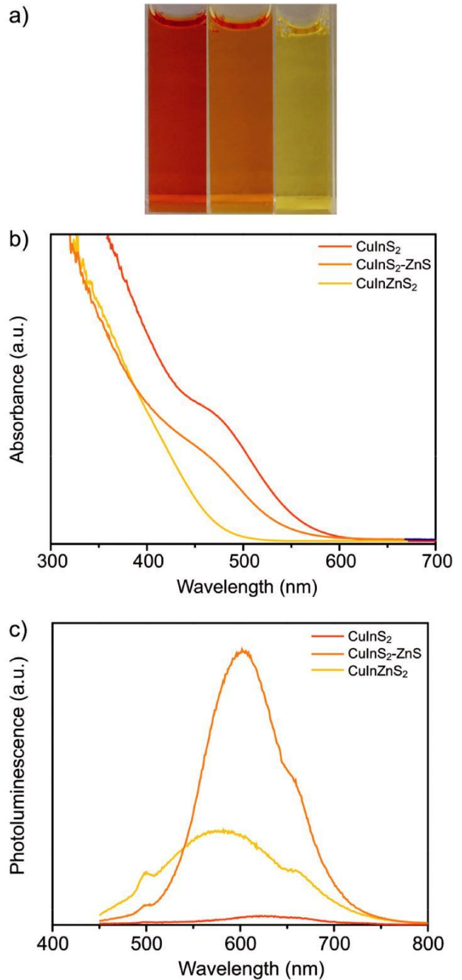
Fig. 6 (a) Images, (b) absorbance spectra, and (c) photoluminescence spectra showing the difference between the original \text{CuInS}_2 quantum dot sol and those materials synthesized with sequential addition versus simultaneous addition of \text{Cu} and \text{Zn} precursors leading to the formation of a \text{CuInS}_2/\text{ZnS} core/shell morphology or a (\text{CuInZn})\text{S}_2 random alloy, respectively.
