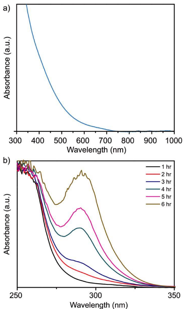
Fig. 1 Absorbance spectra of (a) \text{Cu}_{2-x}\text{S} nanocrystals and (b) In-S complex solutions as a function of time when synthesized by incubation of CSE, L-cysteine and copper acetate or indium nitrate, respectively.
