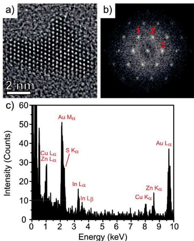
Fig. 7 (a) HRTEM phase contrast image and (b) corresponding FFT of a representative 5 nm (CuInZn) 2 S 2 nanocrystal viewed along the [021 - ] projection. Lattice fitting of planes indicated in the FFT are reported in Table S4.† (c) Representative STEM-XEDS spectrum showing the co-existence of Cu, In, S, and Zn within the single nanoparticle.
