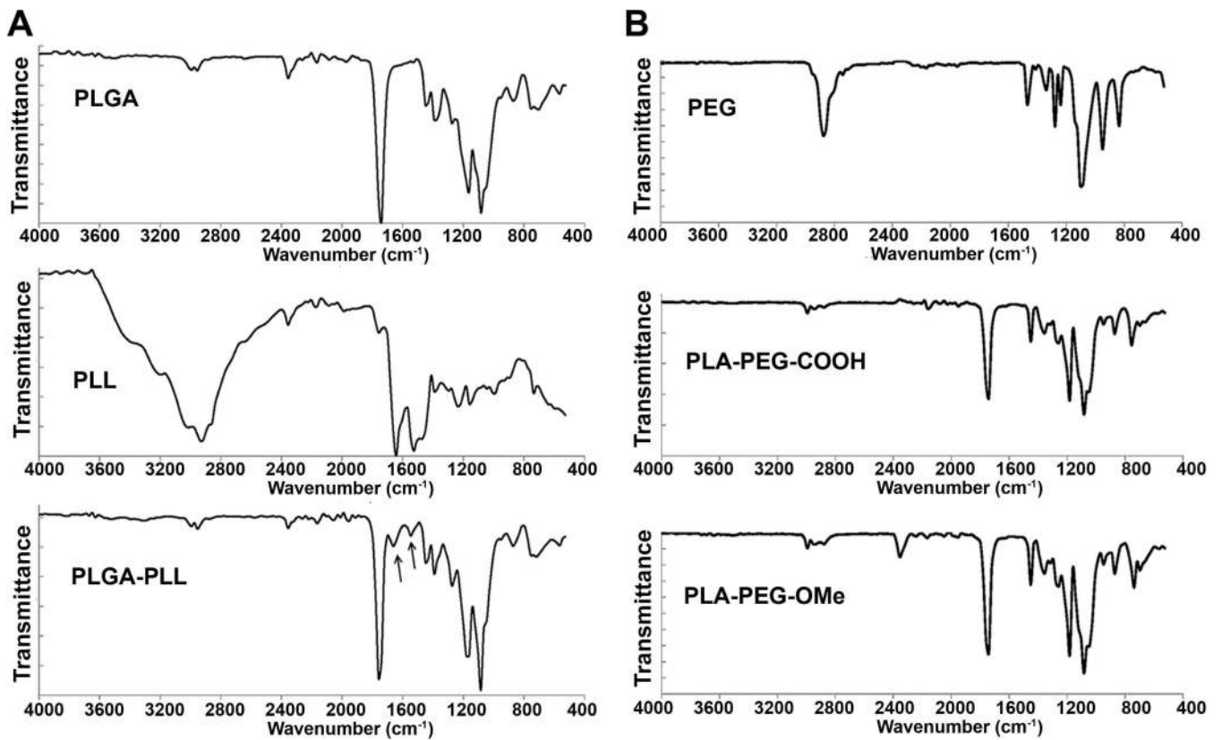
Figure 4. FTIR spectra of synthesized copolymers
