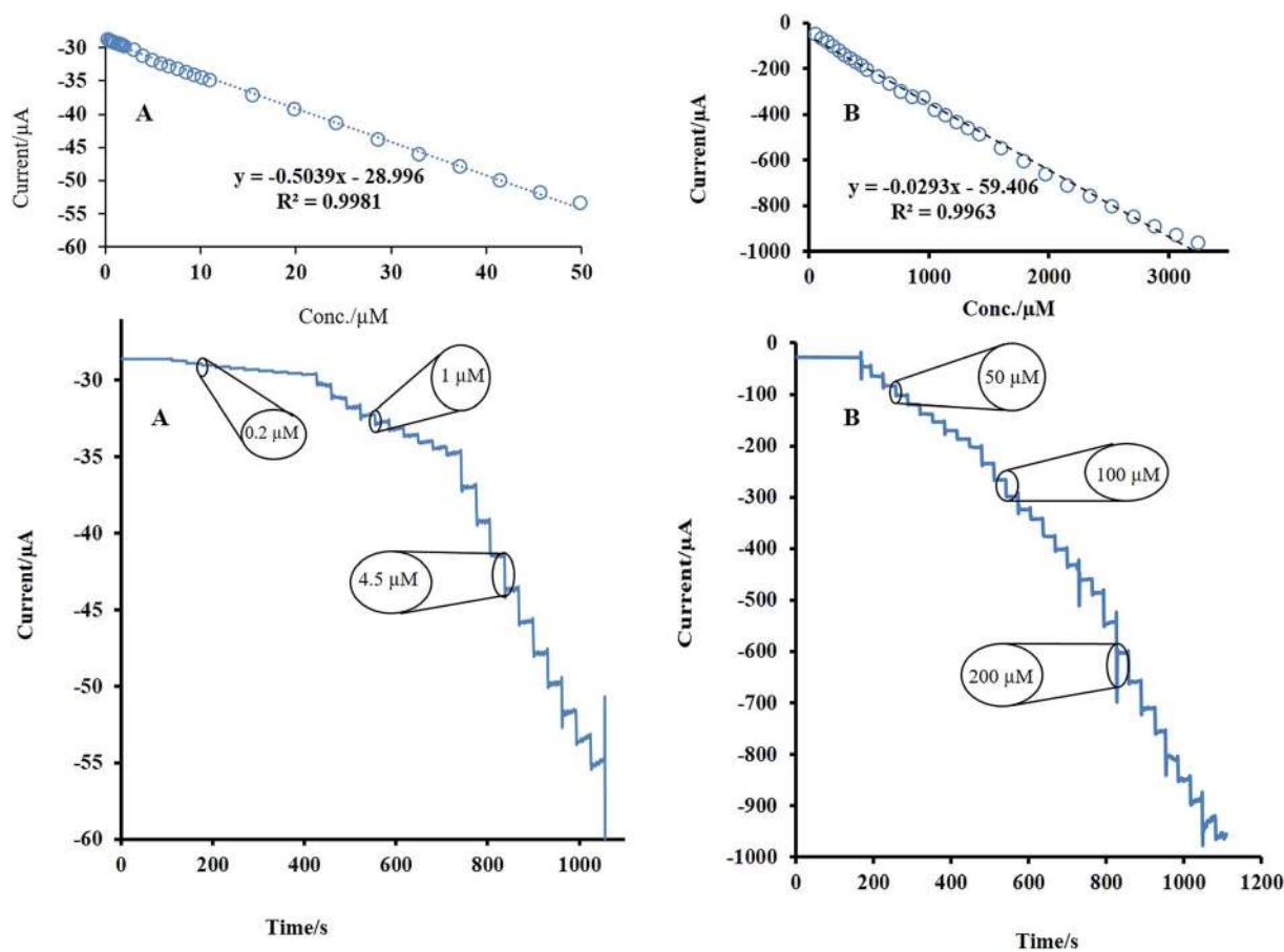
Fig. 6 Amperometric measurements of the \text{H}_2\text{O}_2 at the rotating designed sensor ( 1200 \text{ rpm} ) in 0.1 \text{ M} \text{NaOH} solution for successive addition of various amounts of \text{H}_2\text{O}_2 between 0.2 – 50 \mu\text{M} (A) and 50 – 3240 \mu\text{M} (B) at -0.5 \text{ V} . Insets of (A and B): calibration curve based on the two various ranges of concentration evaluation.
