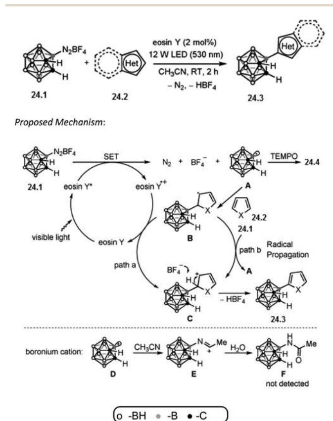
Scheme 24 B–C coupling via a boron-centered carboranyl radical.
