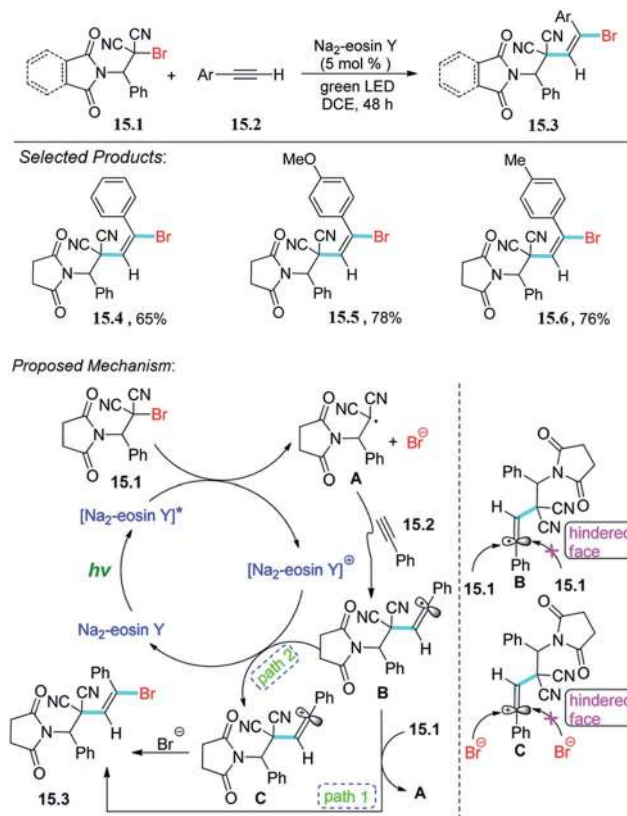
Scheme 15 Difunctionalization of alkynes with alkyl bromides.
