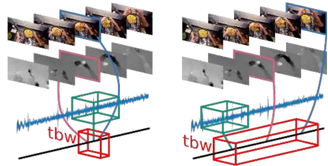
Figure 1: As the width of the temporal binding window increases (left to right), modalities (appearance, motion and audio) are fused with varying temporal shifts.
