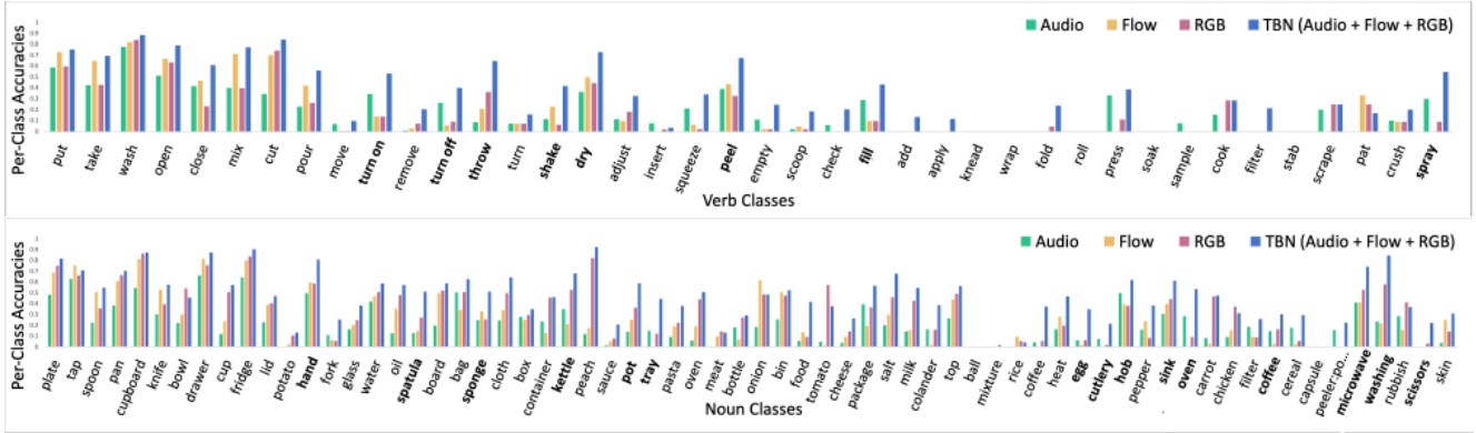
Figure 6: Per-class accuracies for the S1 test set for verbs (top) and nouns (bottom) for fusion and single modalities. We select verb classes with more than 10 samples, and noun classes with more than 30 samples. The classes are presented in the order of number of samples per class, from left to right. For most classes the fusion method provides significant performance gains over single modality classification (largest improvements shown in bold). Best viewed in colour.
