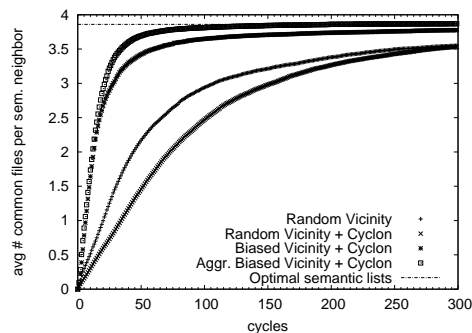
Figure 4. Convergence of sem. views’ quality.
