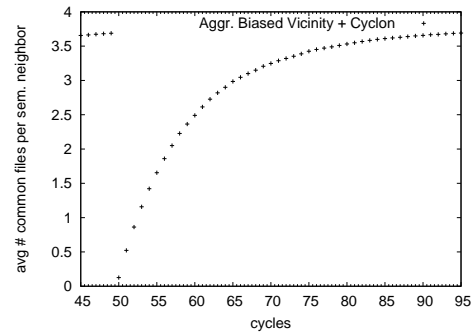
Figure 6. The evolution of semantic views for a sudden change of the interests of all nodes.
