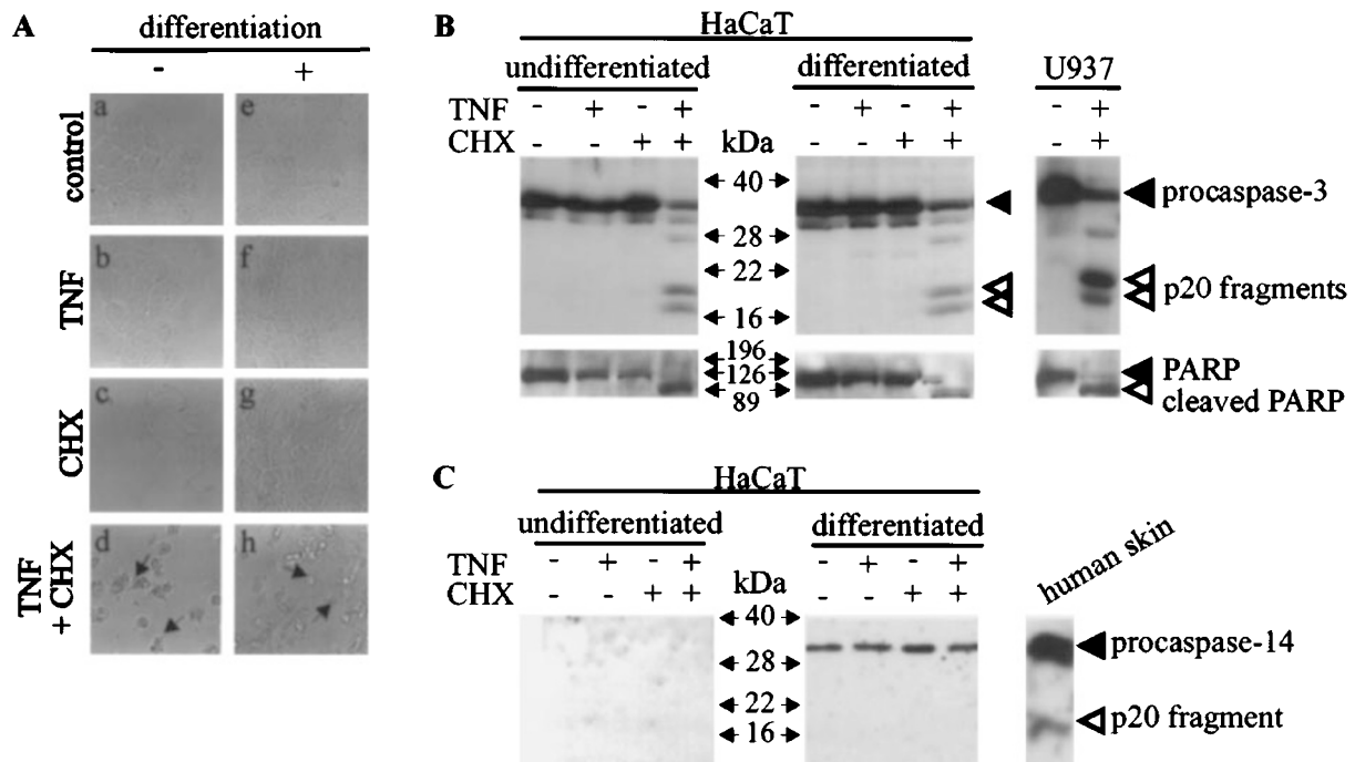
Figure 5 Caspase-14 is not processed in apoptotic conditions. HaCaT cells were grown in normal conditions or induced to differentiate by postconfluent growth. Cells were then treated with TNF (1000 U/ml)+CHX (10 µg/ml) to induce apoptosis. Pictures were taken after 12 h (A); arrows in d and h show apoptotic cells. Lysates were analyzed by immunoblotting for processing of caspase-3 and cleaved PARP (B) as well as caspase-14 (C). Lysates derived from TNF/CHX treated U937 cells were used as control for caspase-3 processing, lysates from human epidermis were applied as control for caspase-14 processing. Filled arrowheads, precursor form; open arrowheads, processed form
