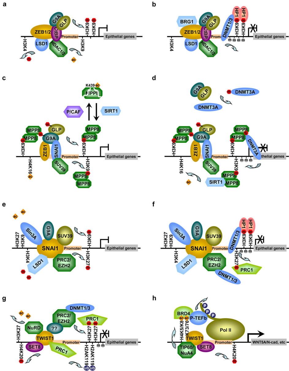
Figure 1. The coordinated transcription regulations mediated by different EMT-TFs and chromatin modifying proteins (A) ZEB1/2 recruit CtBP co-repressor complex in which HDAC1/2 and LSD1 remove histone acetylation and H3K4 methylation respectively whereas G9a/GLP introduce H3K9 methylation. (B) H3K9 methylation marks are recognized by HP1 proteins which further recruit DNMTs for promoter CpG methylation. (C) ZEB1 and SNAI1 recruit multiple H3K9 HMTases to target promoters while the resulting methylation and G9a/GLP self-methylation could target MPP8 for methyl-H3K9 binding. MPP8 protein stability is dynamically regulated by P/CAF- and SIRT1-catalyzed MPP8-K439 acetylation and deacetylation respectively. (D) G9a/GLP also methylate DNMT3A while the resulting K47 methylation facilitates DNMT3A recruitment by MPP8. (E) SNAI1 recruits multiple histone modifying enzymes to remove permissive histone acetylation and H3K4 methylation to introduce
