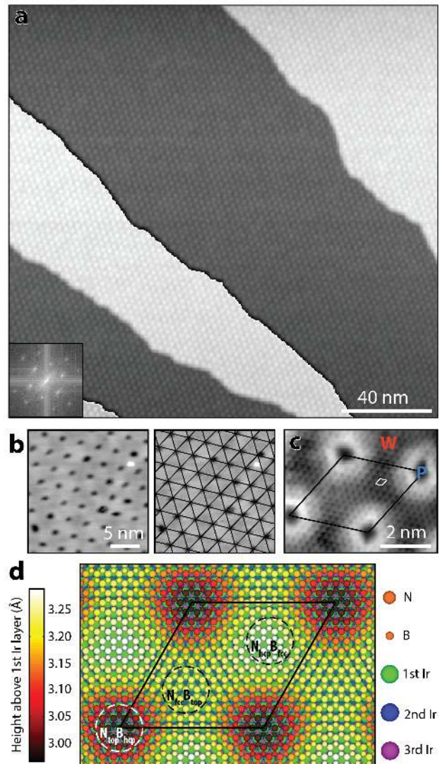
Figure 1. (Color online) Moiré superstructure of hexagonal boron nitride on Ir(111). (a) STM overview image of the sample showing a single h-BN domain extending over four monatomic steps. The black-and-white color scale is adjusted to repeatedly cover the height of two terraces. The inset is a fast Fourier transform of the image, showing six sharp spots indicative of a single rotational moiré domain. (b) Zoom-in on the moiré pattern (left), highlighting its hexagonal periodicity with an overlaid grid (right). (c) Atomically resolved STM image; the moiré and atomic unit cells are indicated in black and white, respectively. Pore and wire regions are marked in the right panel by a blue “P” and a red “W”, respectively. (d) DFT simulation of h-BN on Ir(111). The moiré unit cell as well as regions where B and N atoms occupy high-symmetry positions w.r.t. the Ir lattice are indicated. Feedback parameters: (a) 1.66 V, 0.31 nA; (b) -1.71 V, 0.40 nA; (c) 0.20 V, 3.00 nA.
