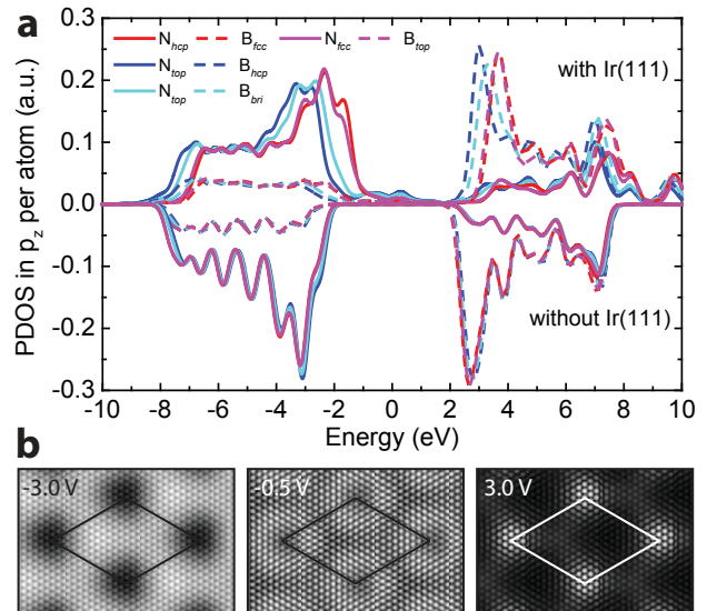
Figure 3. (Color online) Theoretical electronic structure of the h-BN monolayer on Ir(111). (a) The projected density of states of the p_z orbitals of boron and nitrogen resulting from a DFT calculation. (b) Simulated STM images at different bias voltages.
