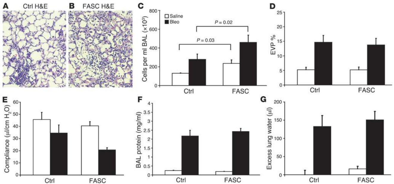
Figure 3 Preserved acute lung injury response in FASC mice. (A and B) Five days after intratracheal bleomycin injury, littermate control (A) and FASC (B) lung sections (original magnification, \times 20 ) were stained with H&E and demonstrated increased inflammation in FASC mice. (C) Cell counts from BAL of littermate control and FASC mice 5 days after intratracheal saline or bleomycin injury. FASC mice had an increased number of cells compared with littermate controls ( n = 4-6 per group). (D) Lung permeability determined by extravasation of intravascular ^{125}\text{I} -albumin into the lungs and expressed as EVP%. FASC and littermate control mice demonstrated similar permeability 5 days after bleomycin injury ( n = 4 per group). (E) Lung compliance ( \mu\text{l}/\text{cm H}_2\text{O} ) was determined from anesthetized and paralyzed ventilated mice. FASC and littermate control mice demonstrated a decrease in compliance 5 days after bleomycin injury. There was a trend toward less compliance in FASC mice after bleomycin injury compared with littermate control mice after bleomycin injury ( P = 0.09 ; n = 4 per group). (F) Total protein concentration (mg/ml) from BAL 5 days after intratracheal saline or bleomycin injury. FASC and littermate control mice demonstrated a similar increase in BAL protein after bleomycin injury ( n = 4-6 per group). (G) Excess lung water (determined as described in Methods) increased similarly in FASC and littermate control mice 5 days after bleomycin injury ( n = 4 per group).
