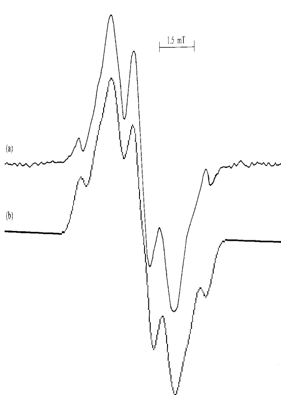
FIG. 2: The EPR spectrum of gamma- irradiated IDAHCl powder, (b) simulation of the spectrum.
