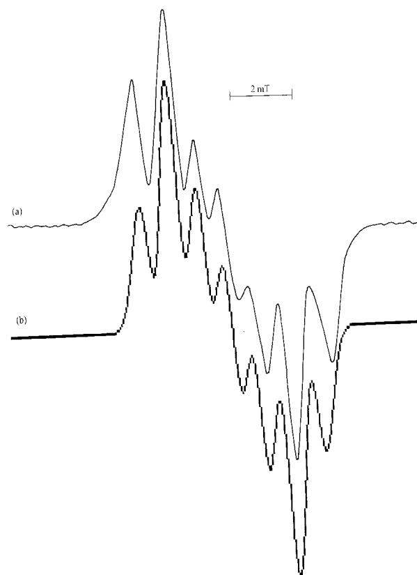
FIG. 3: (a) The EPR spectrum of gamma- irradiated NHIDA powder, (b) simulation of the spectrum.
