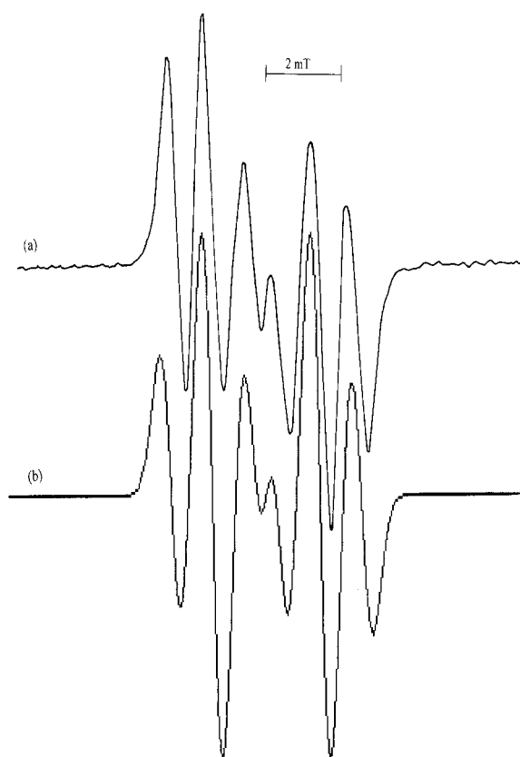
FIG. 1: (a) The EPR spectrum of gamma- irradiated LGHCl powder, (b) simulation of the spectrum.
