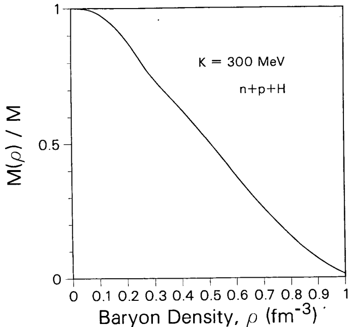
Figure 7: The fraction of mass M(\rho)/M contained in matter at density greater than \rho as a function of baryon density, \rho , for a neutron star at the limiting mass, 1.85M_{\odot} , in the case that K = 300 MeV and the nucleon effective mass in nuclear matter with the same coupling constants is m^*/m = 0.75 at saturation.
