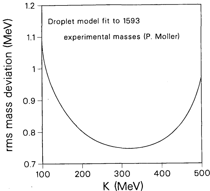
Figure 2: Section of the rms mass deviation of the droplet model fit to atomic mass data as a function of nuclear compression modulus [12,13].
