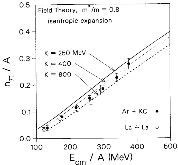
Figure 5: Total pion yields computed in a relativistic nuclear field theory of the fireball following an adiabatic expansion to a freeze-out density of \rho_f = 2\rho_0 from an initial density prescribed by the Rankine-Hugoniot conditions. Data is from [31].
