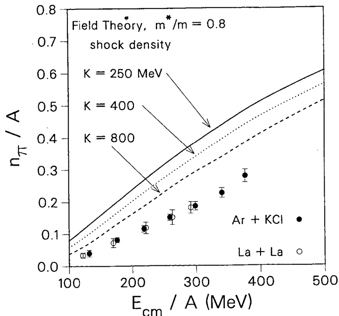
Figure 4: Total pion yields computed in a relativistic nuclear field theory of the fireball at the shock density prescribed by the Rankine-Hugoniot conditions are compared with the data [31].
