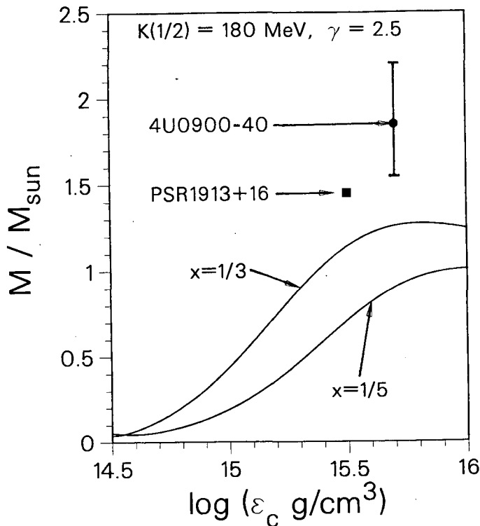
Figure 6: Gravitational mass of neutron stars as a function of central density for the BCK equation of state used in [35] for the value of x = Z/A = 1/3 employed in the reference, and a smaller value, as might be reached in the further evolution of the collapsing matter to the neutron star. The x-coordinate of the two measured masses is not significant since the central density is not measured. The error on the mass of PSR1913+16 measurement is smaller than the data point.
