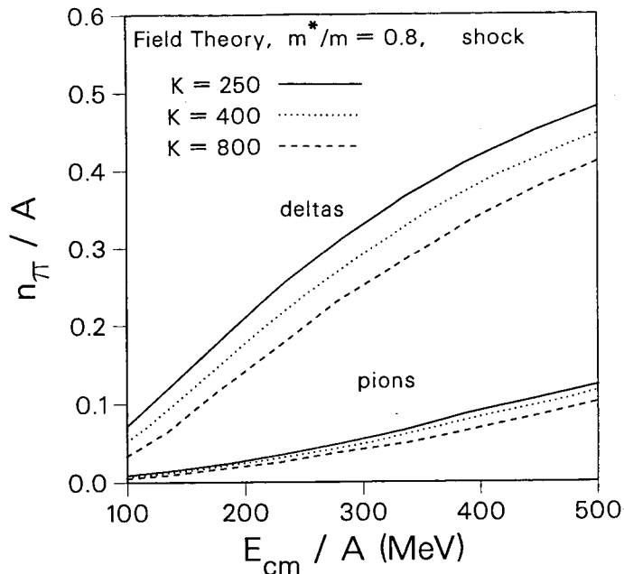
Figure 3: Pion and delta populations in a nuclear fireball described in nuclear field theory, as a function of c.m. energy, at the shock density. Results for three values for K of the corresponding cold nuclear matter are shown.
