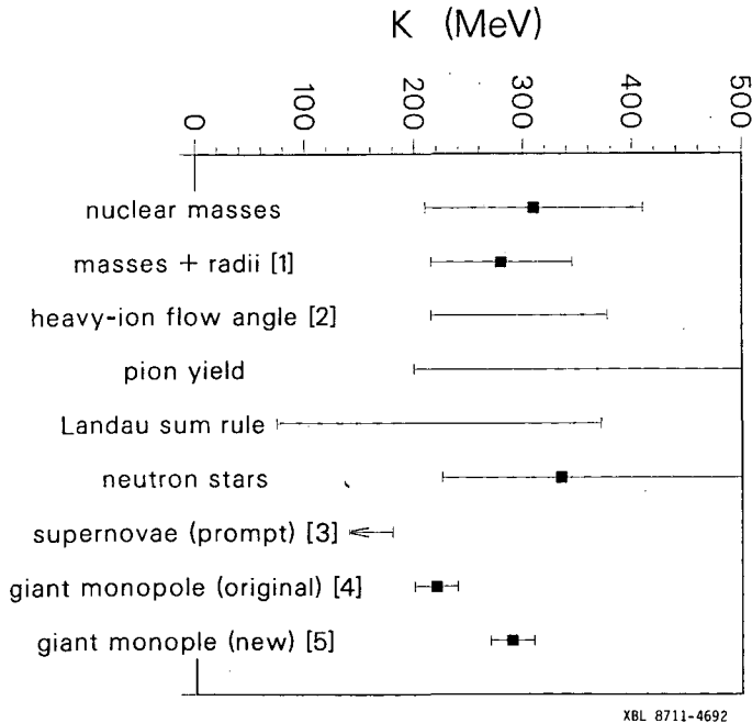
Figure 9: Summary of results for K . The numbered items are taken from other sources referenced as follows. Item numbered 1 is from ref. [48], item 2 from [9], item 3 from [5], item 4 from [3] and item 5 from [50]. Unnumbered items in the figure are from this work.
