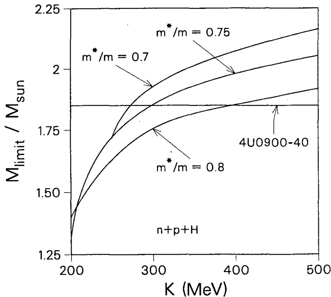
Figure 8: Limiting neutron star mass as a function of compression modulus, of the corresponding cold symmetric matter, are shown for several nucleon effective masses (at saturation density) computed in the relativistic nuclear field theory [42]. Horizontal line represents the most probable mass of neutron star 4U0900-40.
