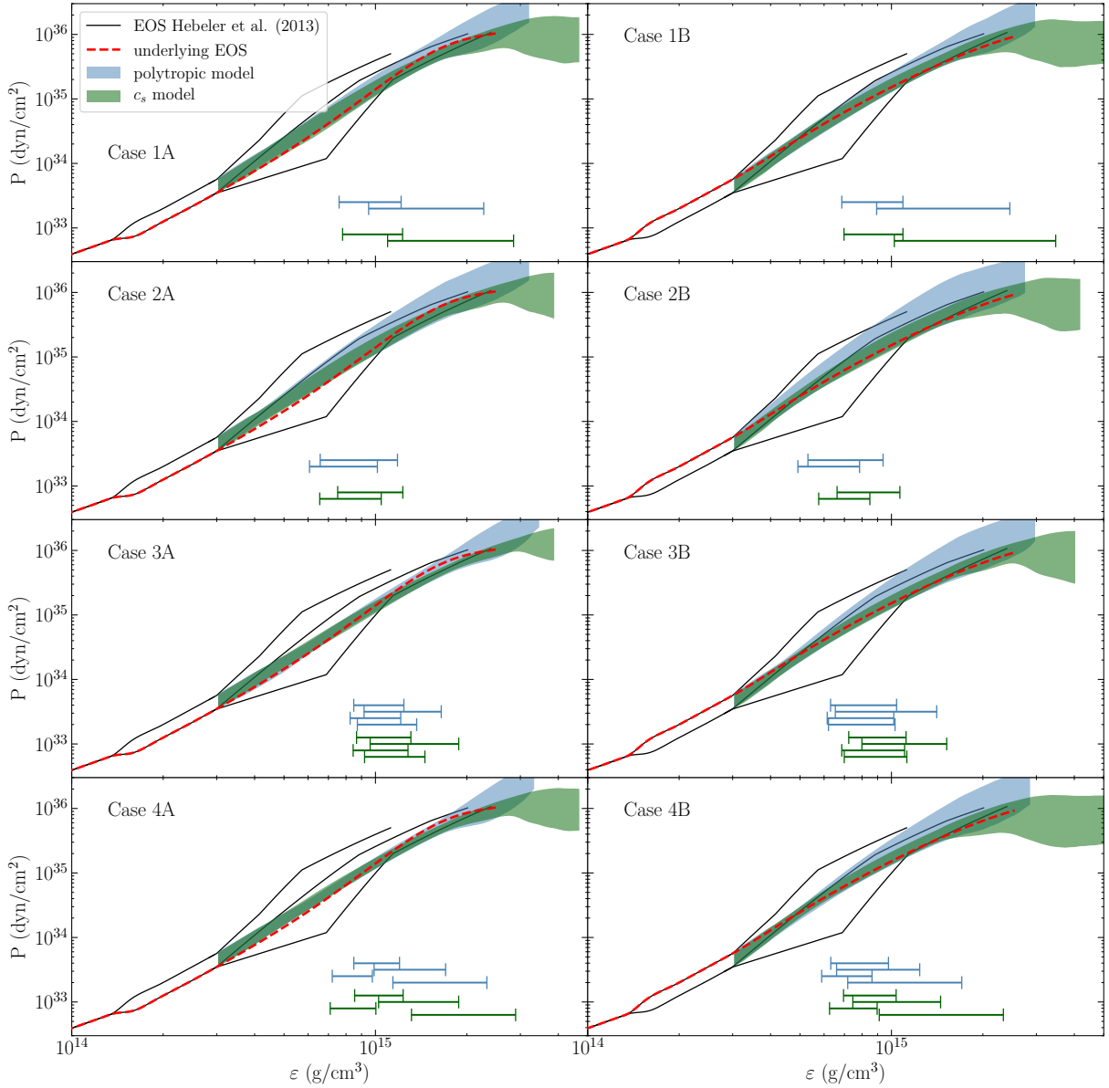
Figure 7. 95% credible regions of the posterior distributions for the EOS for the CS (green) and the PP model (blue). For comparison, the red dashed line represents the underlying EOS used to generate the mass-radius posteriors, while the black EOS are the three representative EOS from Hebel et al. (2013). The narrow features of the green and blue regions are a result of the prior and the likelihood peaking in different regions of parameter space. Especially for Cases A the posterior distribution follows closely the edge of the priors in Fig. 3, indicating that the posteriors are not completely likelihood-dominated. The green and blue horizontal bars in each panel give the 95% confidence interval for the marginalized posterior distribution of the maximal central energy density reached in neutron stars, for the CS and PP model according to the color code.
