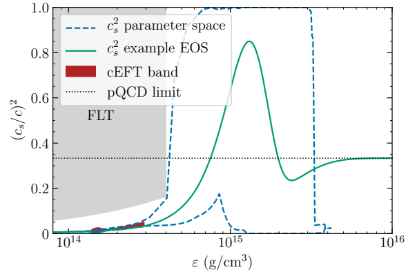
Figure 1. Illustration of the CS parametrization given in Eq. (1). The square of the speed of sound is represented by the solid green line. At the transition density \varepsilon_{\text{cEFT}} the model is matched to the cEFT band, while for very high densities the speed of sound converges from below to the limit of 1/\sqrt{3} that is shown by the black dotted line. The blue dashed outline represents the parameter space that is consistent with the constraints listed in the text. The grey area at low densities represents the excluded region by the Fermi liquid theory (FLT) constraints. Details are given in the text.
