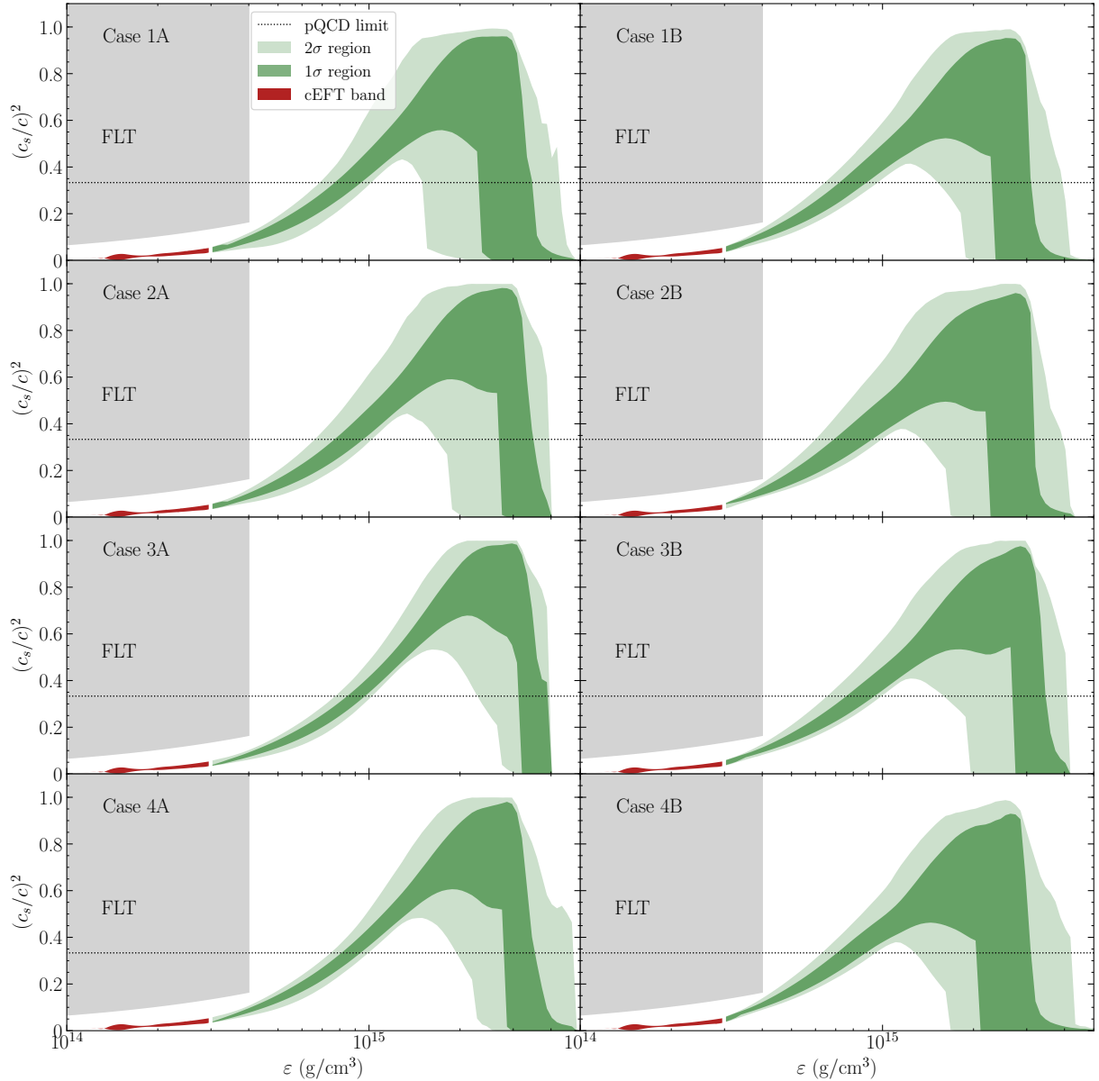
Figure 8. Posterior distributions of the speed of sound in the CS model, where the dark and light green regions represent the joined 68% and 95% credible regions at discrete energy densities. The red area at lower densities gives the speed of sound of the cEFT band calculated by Hebeler et al. (2010) . The dotted line indicates the value 1/\sqrt{3} of the speed of sound in the asymptotic pQCD limit, and the grey area is the excluded region by the Fermi liquid theory (FLT) constraints.
