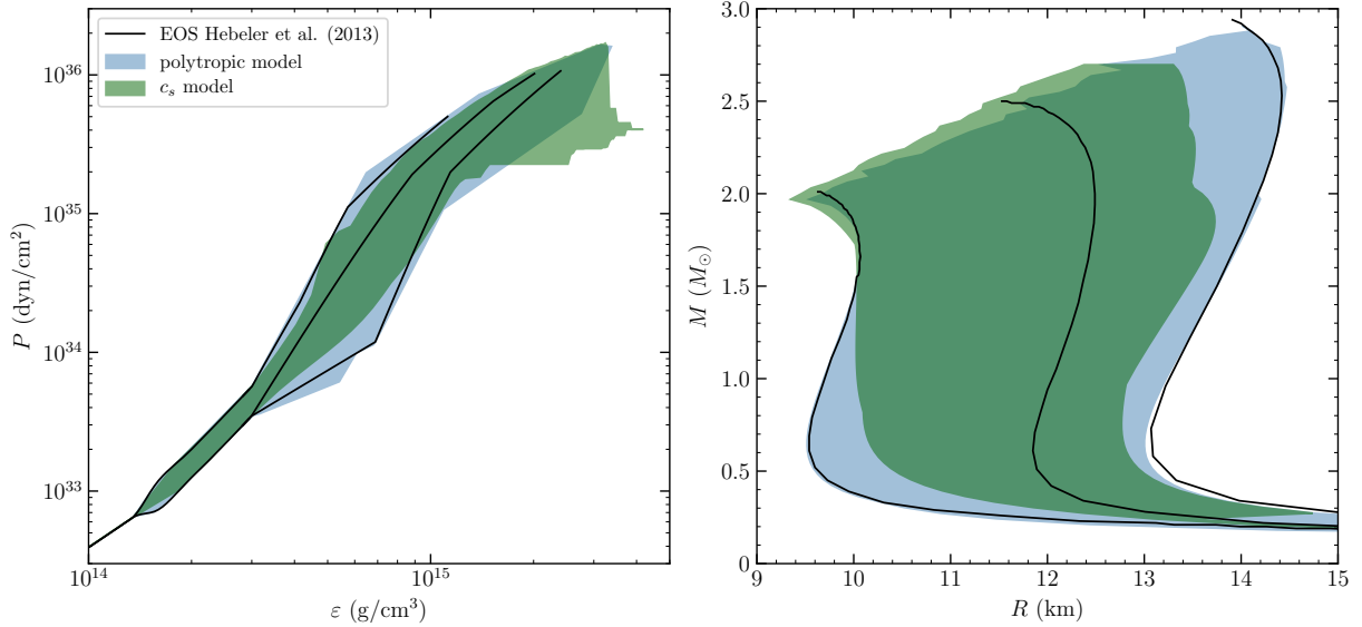
Figure 2. Comparison of the ranges for the EOS (left panel) and mass-radius relations of neutron stars (right panel) based on the PP and CS parametrizations after including all constraints discussed in Section 2.1. The black lines show the three representative EOS of the PP model (Hebeler et al. 2013), the light blue bands show the uncertainty ranges resulting from the PP model and the darker green bands those from the CS model.
