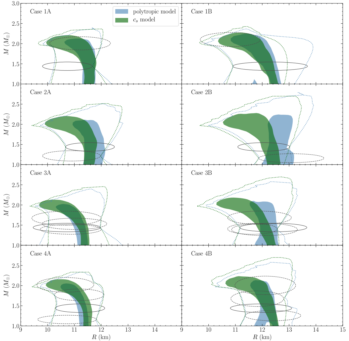
Figure 9. 68% credible regions of the posterior distribution for the mass and radius for the CS (green) and the PP (blue) models. The dotted lines in contrast illustrate the band of all EOS that generate mass-radius curves passing through the 1\sigma contours of the likelihood. These are much wider than the posterior distributions obtained from the Bayesian inference. The elliptical contours of the input mass-radius posteriors for each scenario are shown as well for reference. As in Fig. 4 the solid contour is for PSR J0437–4715 with a known mass of 1.44 \pm 0.07 M_{\odot} , and the dashed ellipses are the other sources.
