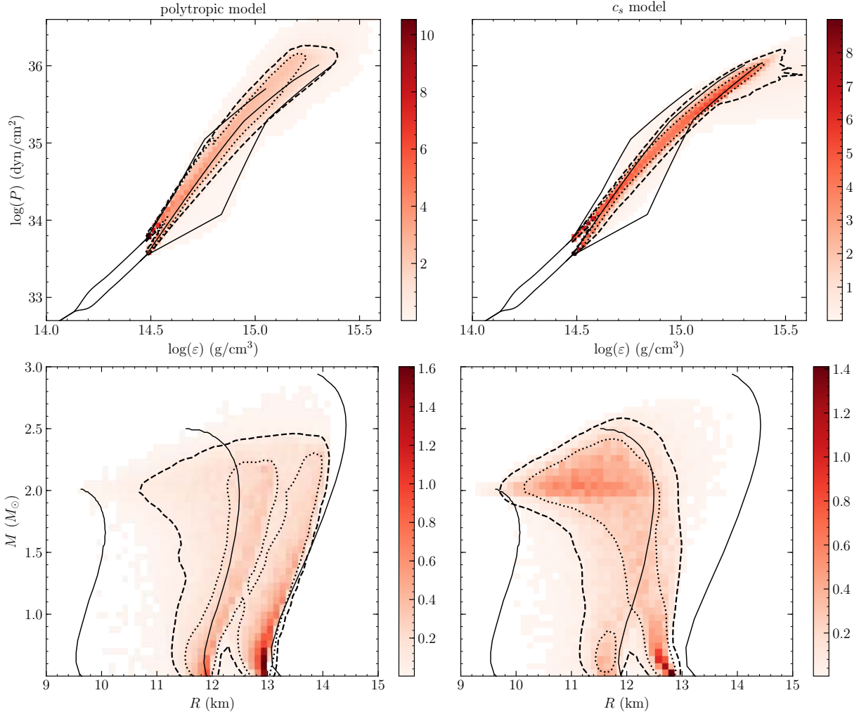
Figure 3. Top: Prior probability distributions transformed to the space of pressure as a function of energy density for the PP (left) and CS parametrization (right panel). The dotted and dashed lines indicate the 68% and 95% credible regions of the distributions, while the solid lines are the representative EOS from Hebeler et al. (2013) . Both prior distributions exhibit a narrow region where most of the probability density is clustered, which falls off steeply towards higher and lower pressures. Bottom: Similar to the upper panels, but now the prior distributions are transformed to the space of mass and radius. We observe that the prior constraints from Section 2.1 result in a higher probability density towards larger radii for both parametrizations. The bimodal feature of the distributions are caused by the way the models have been matched to the lower and upper limit of the cEFT band.
