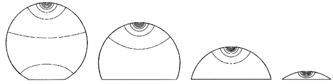
FIG. 4. Four drops of equal radius but different contact angles \theta=154^\circ, 114^\circ, 78^\circ , and 37^\circ . The constant electric potential contours \phi(x,y,z)=c are shown for a vertical slice through each of the four drops. The calculated form factor for each drop is a_{de}(\theta)=\int_{R=1,V=1 \text{ drop}} |\nabla\phi|^2 dv = 0.0592, 0.0609, 0.0617 , and 0.0640 , respectively.
