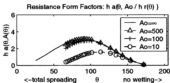
FIG. 10. The constant liquid volume shape factor of Eqs. (32) and (34). If there is no liquid resistance, the form factor is proportional to the liquid/solid area: a(\theta, \infty) = \pi \sin^2 \theta . As the liquid resistance increases ( A_o decreases) the energy stored in the solid falls away from the ideal zero liquid resistance case. Points on the graph above are found by a numerical solution of Eq. (28). When \theta reaches 66^\circ the top of the liquid drop has fallen below the bottom tip of the inserted electrode: this effect can be seen in Fig. 9.
