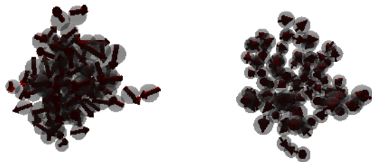
FIG. 1. Left: Visualization of a dense random cluster containing N = 100 nanoparticles prepared as described in Sect. III A. Right: Visualization of a cluster containing N = 100 nanoparticles prepared by DLCA with Q_{dd} = 2 and \varepsilon = 4 as described in Sect. III B.
