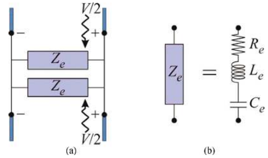
Fig. 4. (a) TL model equivalent network for a periodic surface of dogbone pairs under symmetric (even) excitation. (b) Series resonant RLC circuit representation for the electric mode impedance.
