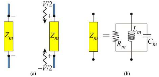
Fig. 5. (a) TL model equivalent 2-port network for a periodic surface of dogbone pairs under antisymmetric (odd) excitation. (b) Parallel resonant RLC circuit representation for the magnetic mode impedance.
