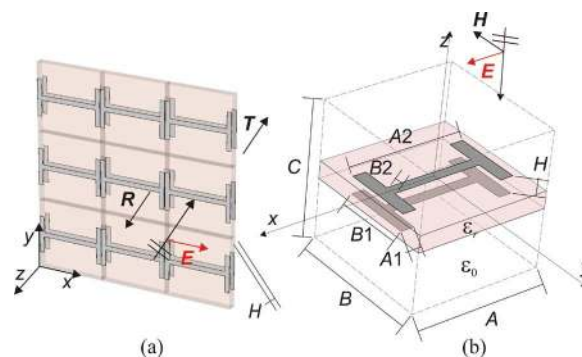
Fig. 1. (a) Perspective view of a metalayer (one layer of the metamaterial) formed by a periodic arrangement of pairs of dogbone-shaped conductors printed on a dielectric substrate. (b) Metamaterial elemental particle (unit cell) with geometrical parameters quoted. The polarization of the incident electric field is along the x-direction.
