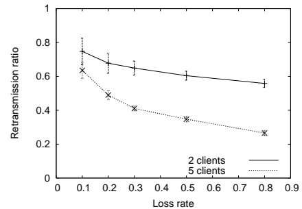
Figure 17: Compare retransmission mechanisms for unicast under a varying loss rate, where only packets destined to the receivers are dropped.
