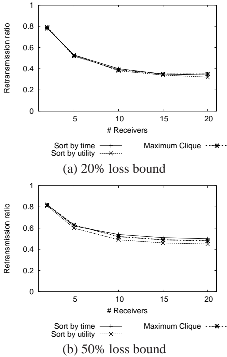
Figure 6: Multicast comparison under a varying number of receivers with heterogeneous Bernoulli losses.
