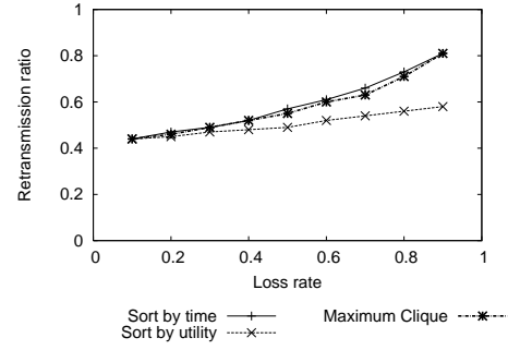
(b) 5 receivers
