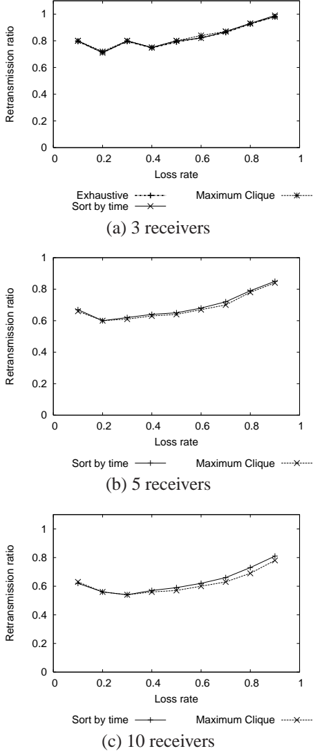
Figure 9: Unicast comparison under a varying loss rate with homogeneous Bernoulli losses.
