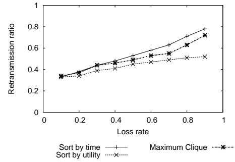
(c) 10 receivers
