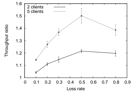
Figure 15: Compare throughput against the basic scheme for multicast under a varying loss rate.
