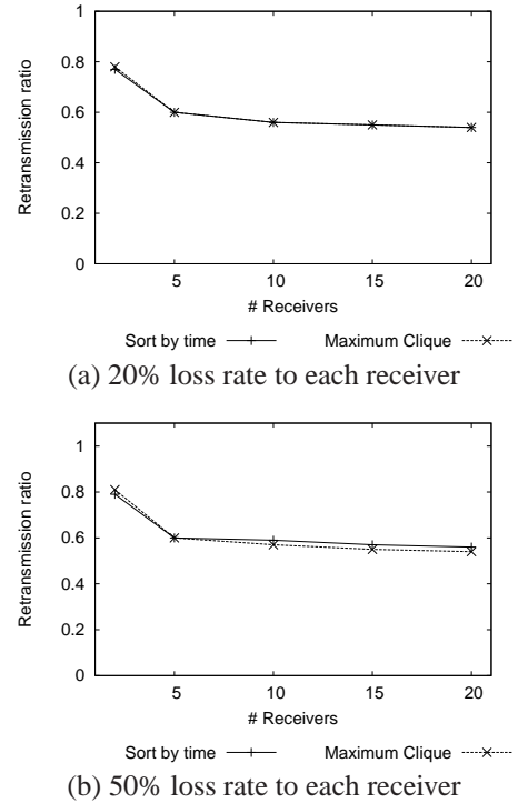
Figure 8: Unicast comparison under a varying number of receivers with homogeneous Bernoulli losses.
