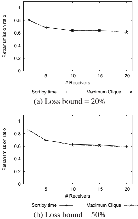
Figure 11: Unicast comparison under a varying number of receivers with heterogeneous Bernoulli losses.
