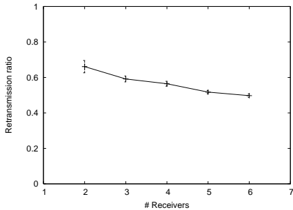
Figure 14: Multicast experiment results under a varying number of clients.
