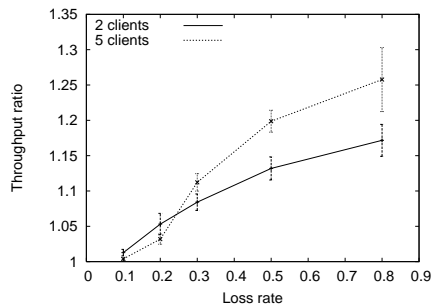
Figure 19: Compare throughput against the basic scheme for unicast under a varying loss rate.
