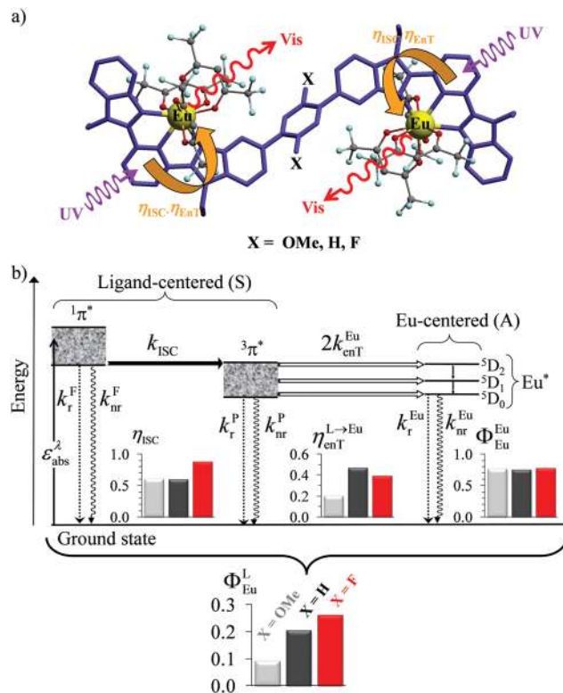
Fig. 6 (a) Molecular structures and (b) simplified Jablonski diagram for [(hfac) 3 Eu] 2 Lu(hfac) 3 showing the indirect ligand-centred triplet-mediated sensitization mechanism of the two Eu 3+ activators. The photophysical processes are described by first-order rate constants: k_r^F = ligand fluorescence, k_{nr}^F = ligand internal non-radiative conversion, k_r^P = ligand phosphorescence, k_{nr}^P = non-radiative relaxation from the ligand triplet state, k_r^{\text{Eu}} = emission of Eu*, k_{nr}^{\text{Eu}} = nonradiative decay of Eu*, k_{\text{ISC}} = ligand intersystem crossing, and k_{\text{en.tr.}}^{\text{Eu}} = ligand-to-metal energy transfer. Efficiencies of intersystem crossing ( \eta_{\text{ISC}} ), of energy transfer ( \eta_{\text{en.tr.}}^{\text{Eu}} ), of intrinsic quantum yield ( \Phi_{\text{Eu}}^{\text{L}} ), and global quantum yield ( \Phi_{\text{Eu}}^{\text{A}} ) characterize the antenna effect (solid-state, 293 K). Adapted from ref. 17b.
