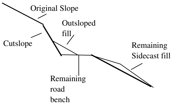
c Partial Outslope
