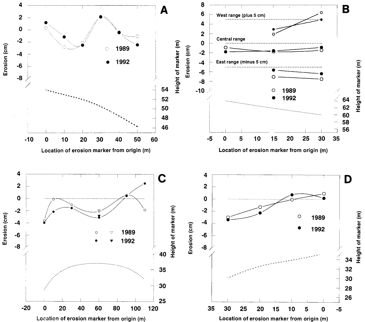
FIG. 9. Surface erosion as given by the alterations in the distance between the tops of permanent markers and the surface of the ground. These data are compared to hill profiles (lower curves) which are given by plots of the heights of markers, in metres, above reference point B. Graphs A, B, C and D display readings at ranges A, B, C and D respectively. Negative values indicate erosion. The triangular points in 9C are for a marker displaced 10 m at right angles to the line of the main C array.
