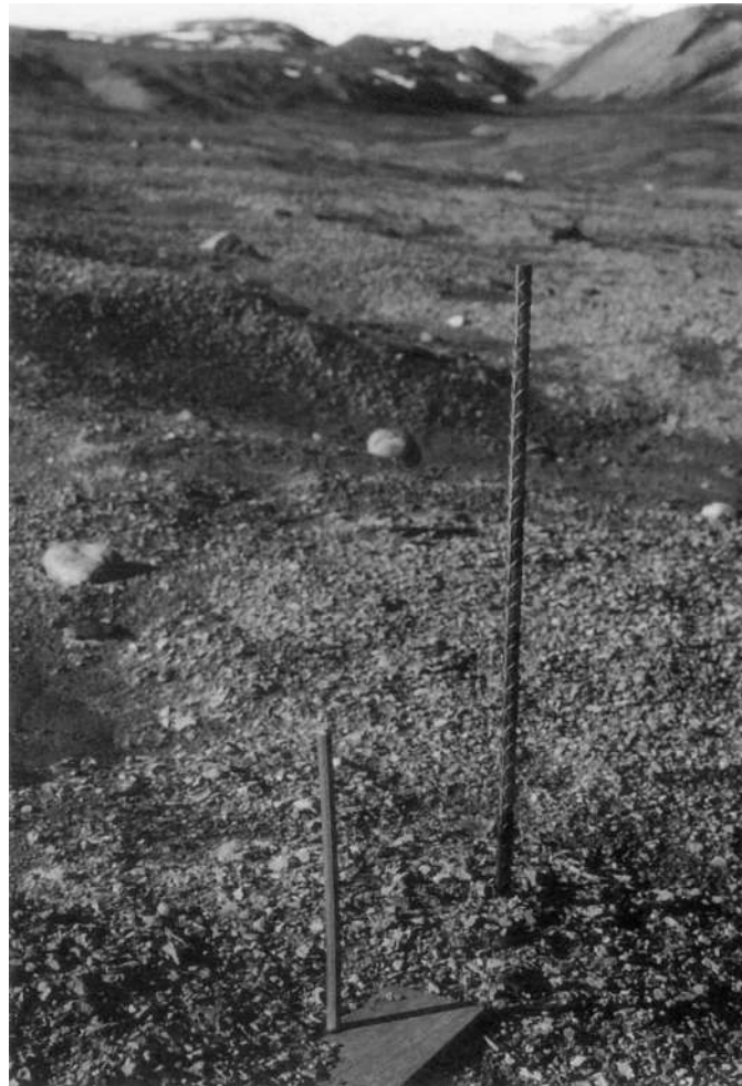
FIG. 6. A floating and a permanent marker. The partially covered floating marker is direct evidence of accretion.
