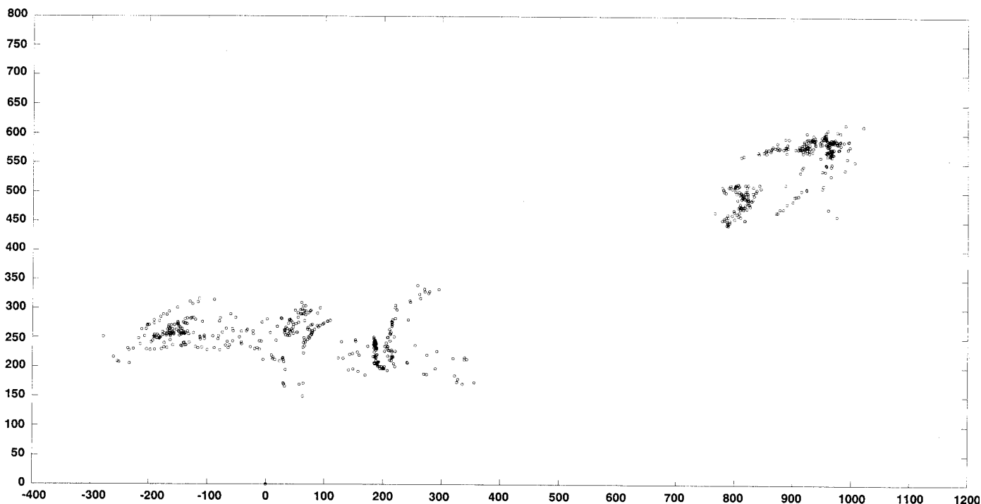
FIG. 8. Cumulative plot of stumps surveyed in 1988, 1989 and 1992. The horizontal axis follows the baseline joining trig points B (0,0) and A (613,0). All distances are in metres.
