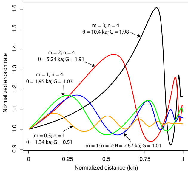
Figure 4. Computed normalized erosion rate ( \frac{\partial h}{\partial t}/U ) as a function of the normalized distance ( x/L ) along the river profile for a forcing at P = 100 ka and for various values of the exponents m and n ; for each run we indicate the value of the computed time lag, \theta , and gain, G .
