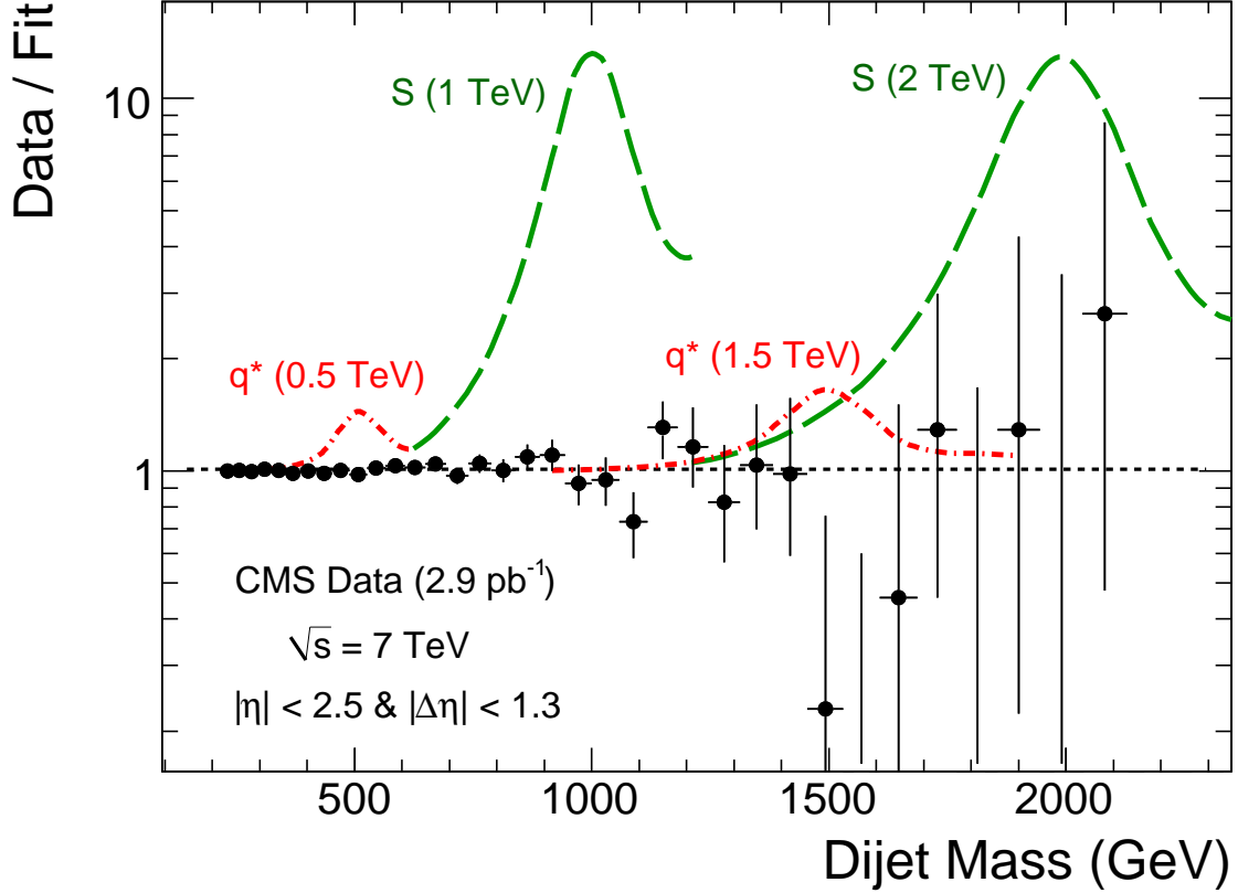
Figure 2: Ratio (points) between the dijet mass data and the smooth fit, compared to the simulated ratios for excited quark signals (dot-dashed) and string resonance signals (long-dashed) in the CMS detector. The errors are statistical only.
