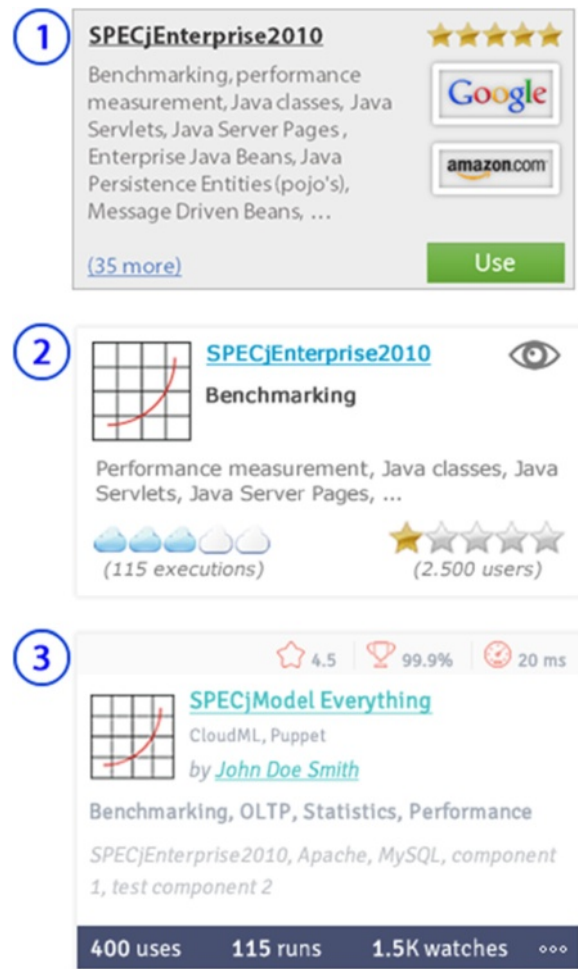
Fig. 11 Evolutionary design of the application model overview panel
