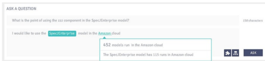
Fig. 10 Automatic provision of context-sensitive assistance when available
