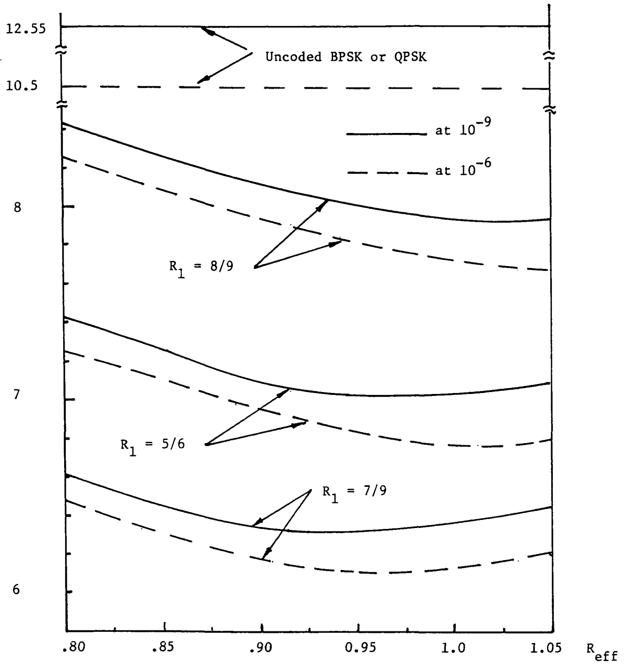
Fig. 5.8 E_b/N_0 required to achieve P_b = 10^{-6} and 10^{-9} vs. R_{eff} for Example 3.2 with 16-state PTVTCs as inner codes (simulation).
