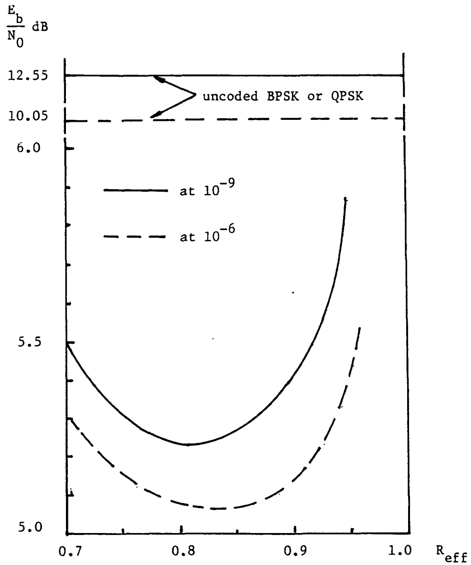
Fig. 6.2 E_b/N_0 required to achieve P_b = 10^{-6} and 10^{-9} vs. the overall effective information rate R_{eff} for Example 3.3 with Ungerboeck's 16-state R_1 = 2/3 coded 8PSK as inner code (simulation).
