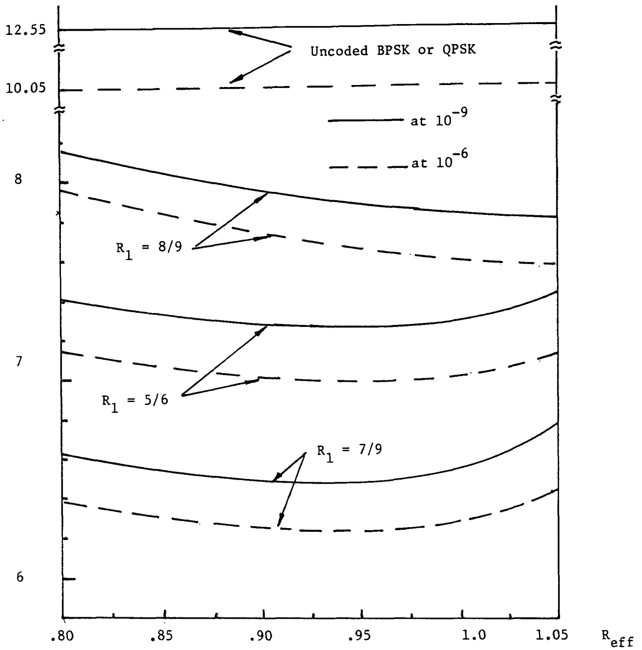
Fig. 5.7 E_b/N_0 required to achieve P_b = 10^{-6} and 10^{-9} vs. R_{eff} for Example 3.2 with 4-state PIVTCs as inner codes (simulation).
