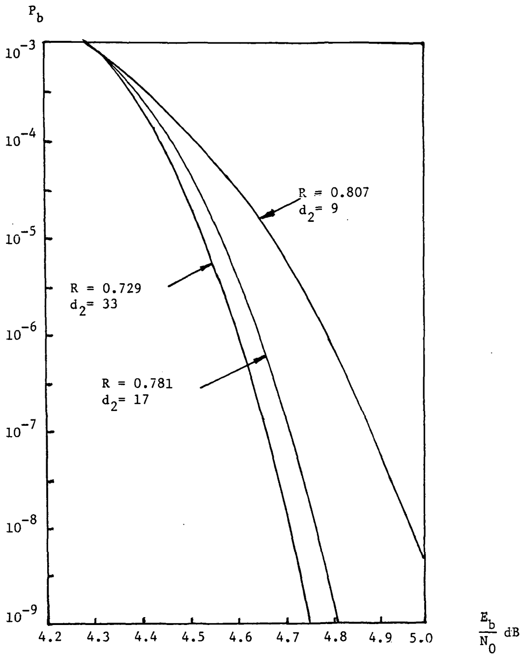
Fig. 4.2 Performance of Example 3.1 (simulation) with R_1 = 5/6 punctured convolutional code as inner code.
