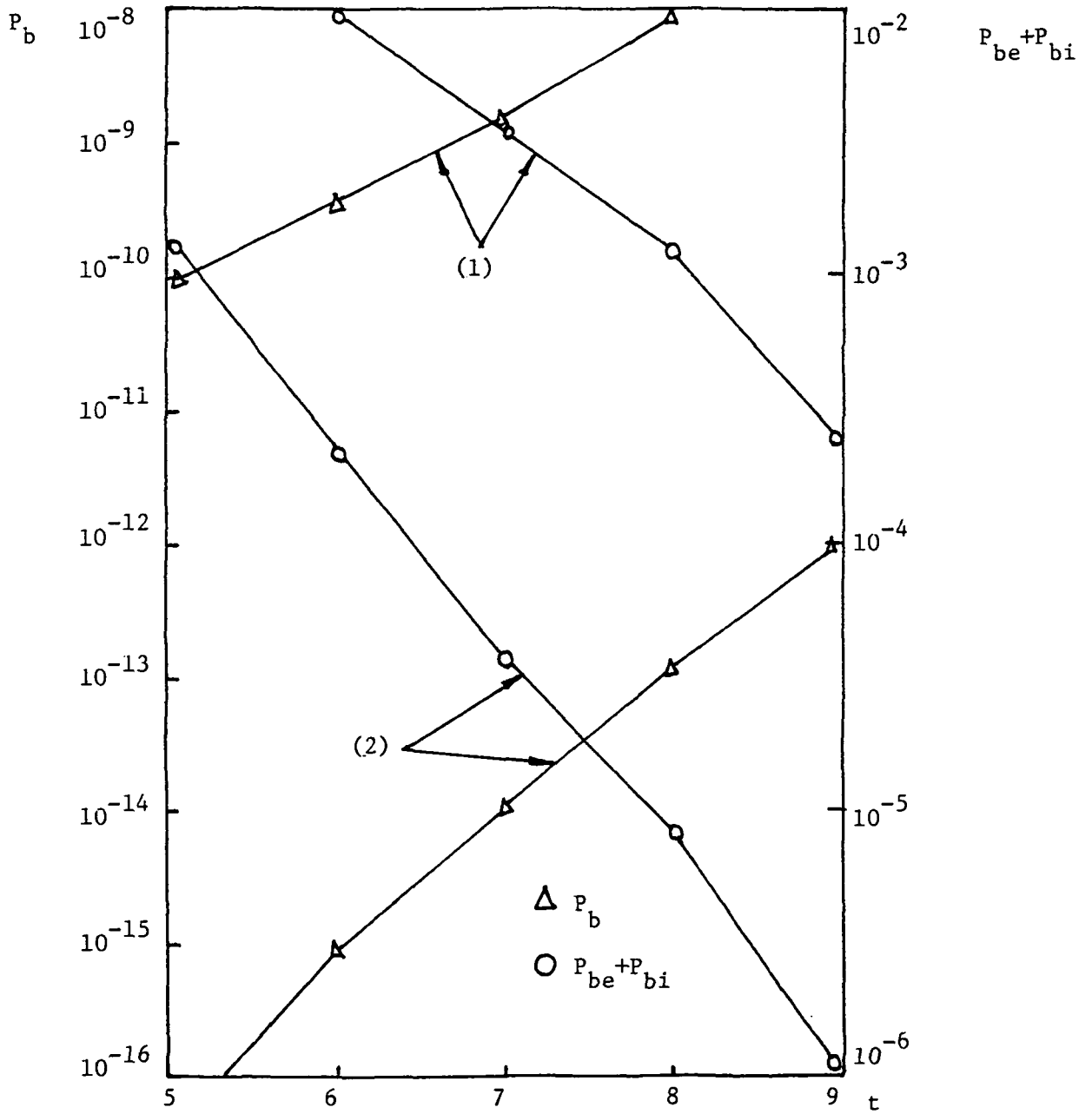
Fig. 16 Code performance of Example 5.3 (simulation) with 16-state R_1=2/3 coded 8PSK inner code, and B=4 , T'=0.3 , T_{es}=10 , d_2=26 , R_{eff}=0.9 . (1) E_b/N_0=5.07 dB ( P_b=1.11 \times 10^{-6} in scheme 1); (2) E_b/N_0=5.45 dB ( P_b=5.3 \times 10^{-10} in scheme 1).
