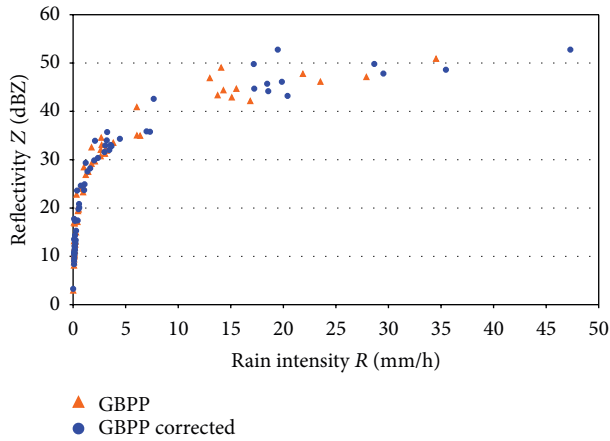
FIGURE 13: Z-R relationship calculated with the sampling area uncorrected (GBPP) and corrected (GBPP corrected).
