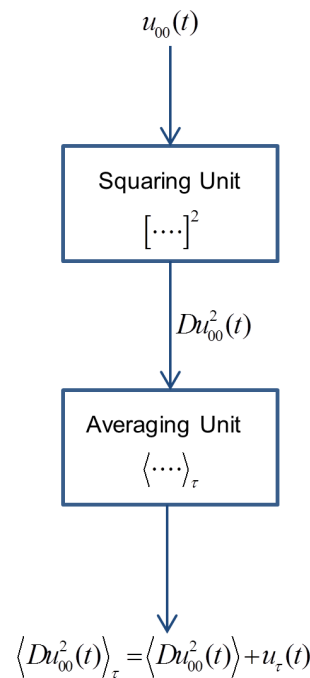
Figure 3. Illustration of the measurement process at 00. D is calibration coefficient of the squaring device to provide a Volt unit with the correct numerical value for the squaring operation. doi:10.1371/journal.pone.0081103.g003
