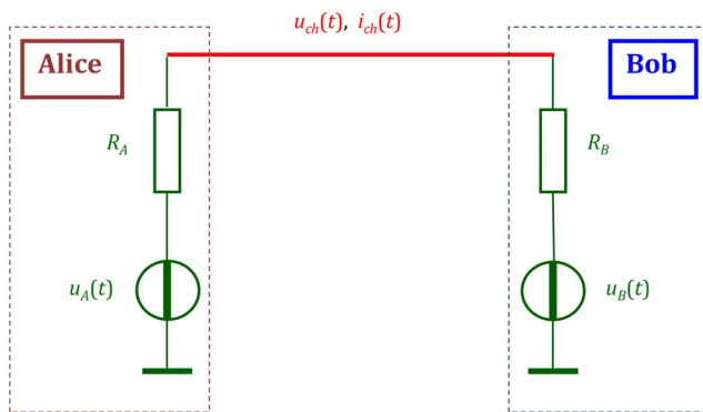
Figure 1. Outline of the core KLJN secure exchange scheme [2–4,28] without the defense elements against active (invasive) attacks or attacks utilizing non-ideal components and conditions. R_A, u_A(t), R_B, and u_B(t) are the resistor values and noise voltages at Alice and Bob, respectively. u_{ch}(t) and i_{ch}(t) are channel noise voltage and current, respectively. doi:10.1371/journal.pone.0081103.g001
