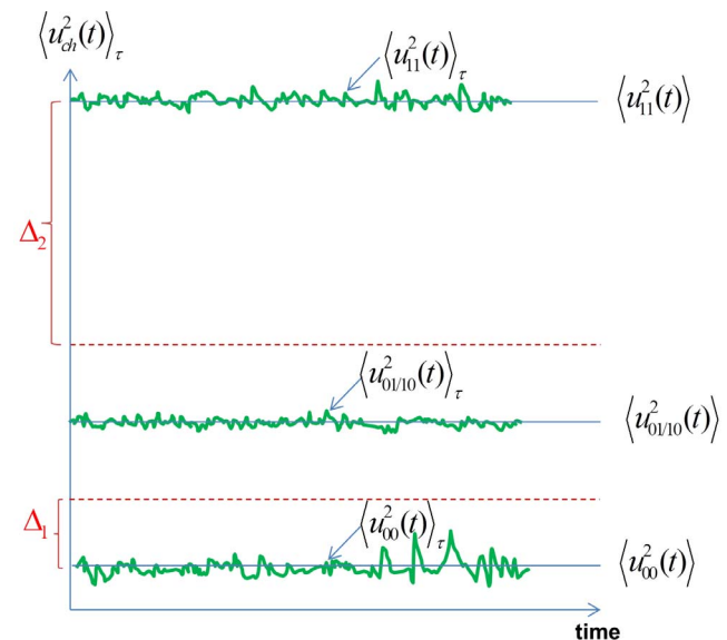
Figure 2. Illustration of the fluctuations of the finite-time mean-square voltage levels around their exact value and thresholds for interpretation (the scale is arbitrary). \langle u_{11}^2(t) \rangle_\tau , \langle u_{01/10}^2(t) \rangle_\tau , \langle u_{00}^2(t) \rangle_\tau are the measured mean-square channel noise voltages at the 11, 01/10 and 00 bit situations, respectively. The solid lines with the quantities in \langle \rangle represent ideal (infinite-time) averages. For the sake of simplicity we assume R_0 = R and, R_1 = \alpha R with \alpha > 1 . doi:10.1371/journal.pone.0081103.g002
