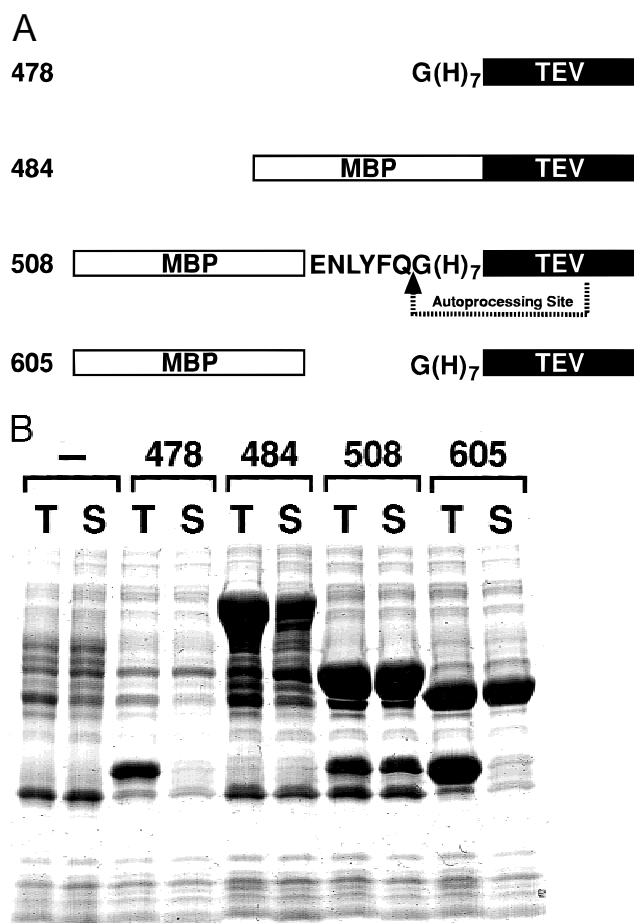
Fig. 3. Proper folding of TEV protease is promoted by fusion to MBP. A: Schematic illustration of the proteins produced by four different TEV expression vectors (not to scale): 478, His-tagged TEV protease; 484, MBP-TEV fusion protein; 508, self-processing MBP-TEV fusion protein; 605, separate MBP and His-tagged TEV protease domains synthesized from a single, dicistronic mRNA. B: Samples of the total and soluble intracellular protein fractions from cells containing the TEV expression vectors in A were prepared as described (see Materials and methods) and analyzed by SDS-PAGE.
