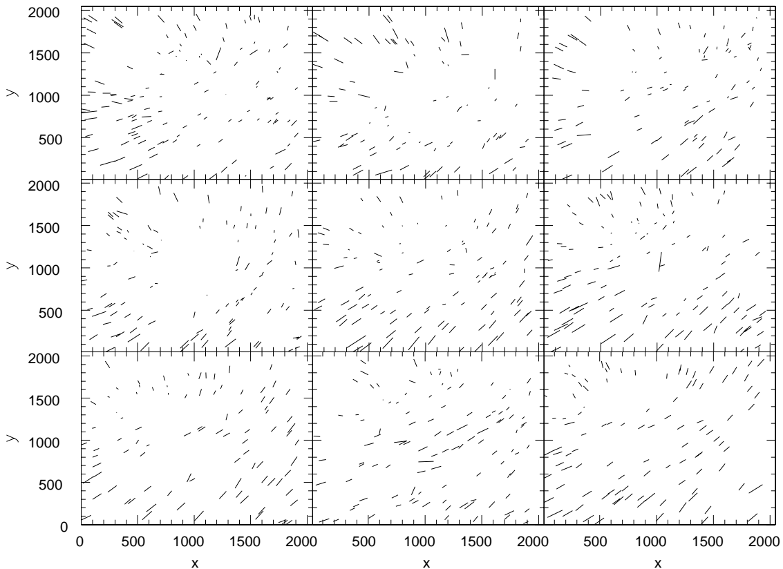
Fig. 12. Nine consecutive EIS images showing the stability of the PSF anisotropy with time
