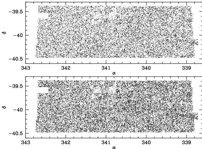
Fig. 15. Distribution of stars detected in the even frames covering patch A at magnitudes brighter than I = 20 (12355 objects, upper panel) and I = 21 (18529, lower panel). Objects with a stellarity index > 0.5 were classified as stars. Note the two bad frames in the upper part of the patch, yielding nearly empty regions. As pointed out in the text this region is usually discarded from the analysis
