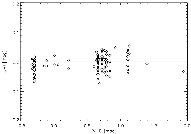
Fig. 4. Relation between the EIS and Johnson-Cousins system as a function of Johnson-Cousins color. Shown are all the standard stars observed under photometric conditions in the period July 97-January 98
