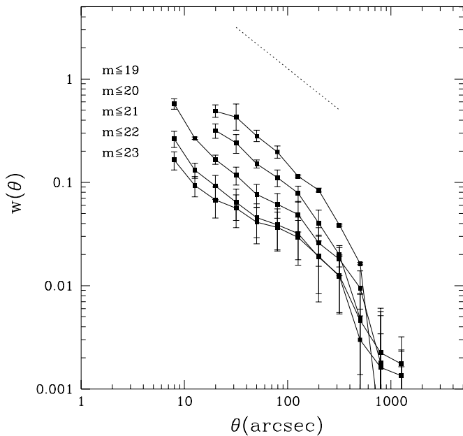
Fig. 28. Mean value of the angular correlation function measured for 6 sub-catalogs covering the whole patch. The error bars are the standard deviations calculated between these subsamples, and are therefore an estimate of the cosmic variance on the corresponding scales. The dotted line represents a power-law with a slope of -0.8
