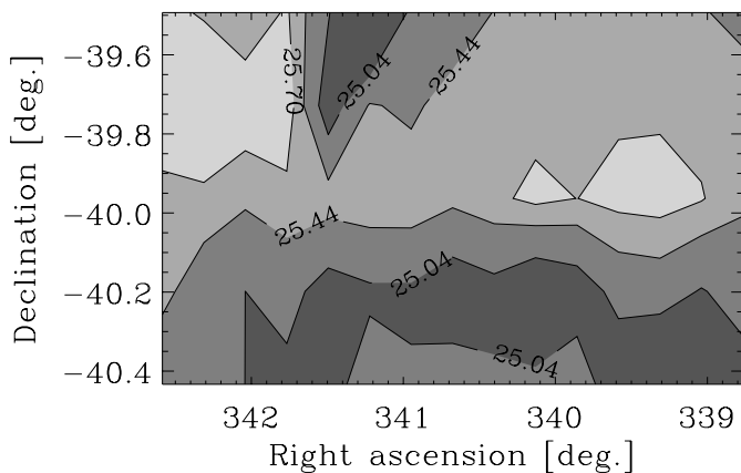
Fig. 8. Two-dimensional distribution of the computed 1\sigma limiting isophote for the accepted even frames for patch A. Contours refer to 25, 50 and 75 percentiles of the distribution
