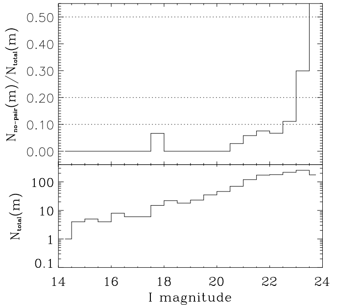
Fig. 20. Top panel: ratio of the number of objects found in a single-frame but not in the the coadded catalog of the reference field and total number of objects in the corresponding single-frame catalog. At I \sim 22.5 there are 10% false objects and at I \sim 23 there are 20% spurious detections. Bottom panel: total number counts in the single-frame catalog
