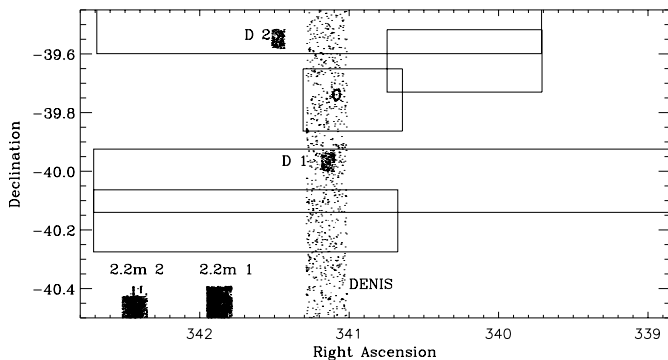
Fig. 5. Distribution of frames obtained at the 2.2 m and the 0.9 m Dutch (D) telescopes at La Silla within the covered region of patch A. Also shown is a part of a DENIS strip that crosses the field. The open rectangles represent regions containing EIS tiles observed under photometric conditions
