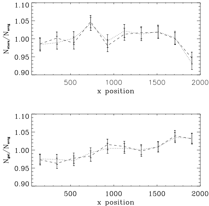
Fig. 17. The uniformity of the detections in the east-west direction. The top panel shows the detected stars brighter than I = 21 for a stellerity index \geq 0.75 (dotted line) and stellerity index \geq 0.5 (dashed line). For fainter magnitudes the classification breaks down. The bottom panel shows the detected galaxies brighter than I = 21 stellerity index < 0.75 (dotted line) and stellerity index < 0.5 (dashed line). It is seen that the star counts show a dip at the “right” edge of the chip, and a corresponding increase in the galaxy counts. This feature is attributed to the image distortions, see text for details
