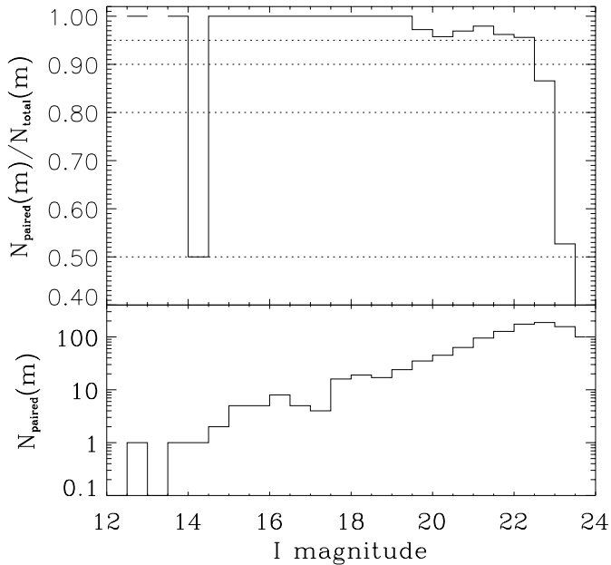
Fig. 19. Top panel: Completeness of the single-frame catalogs as determined from the comparison with the reference field. The plot shows the ratio between the number of objects found in both the coadded image and a single frame and objects found in the coadded image as a function of magnitude. The figure shows that at I \sim 23 the single-frame catalogs are 80% complete. Bottom panel: The number of paired objects, to give an idea of the statistical errors in the comparison
