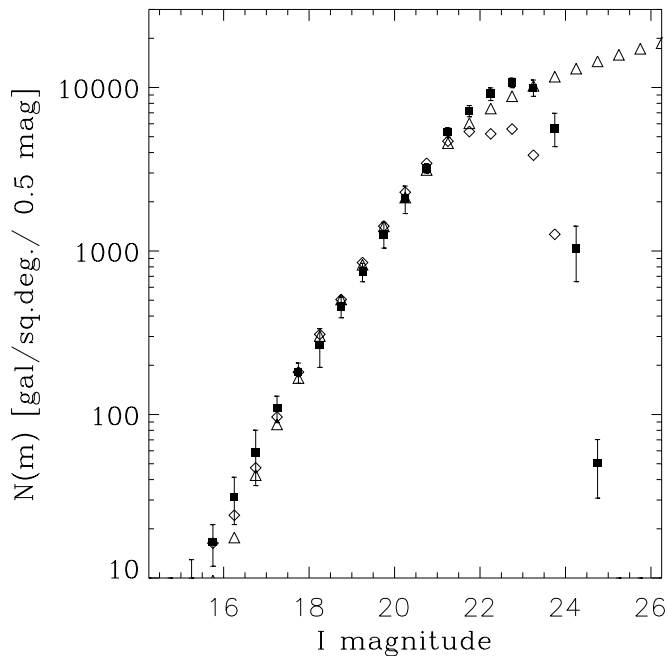
Fig. 24. The EIS galaxy counts (filled squares) with 1\sigma error bars compared to the galaxy counts derived by Lidman & Peterson (1996) (triangles) and Postman et al. (1996) (diamond). The data from the other authors have been converted to the Johnson-Cousins system
