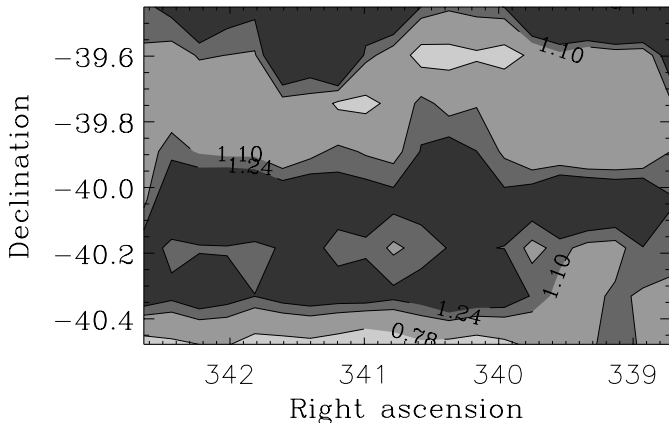
Fig. 7. Two-dimensional distribution of the seeing as measured on the I -band images for patch A for all the accepted even frames. Contours refer to 25, 50 and 75 percentiles of the distribution
