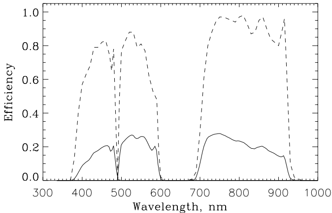
Fig. 1. Transmission curves for the EIS filters (dashed lines) and total system throughput including the contribution from the filters, telescope and camera optics, and the detector (solid lines)
