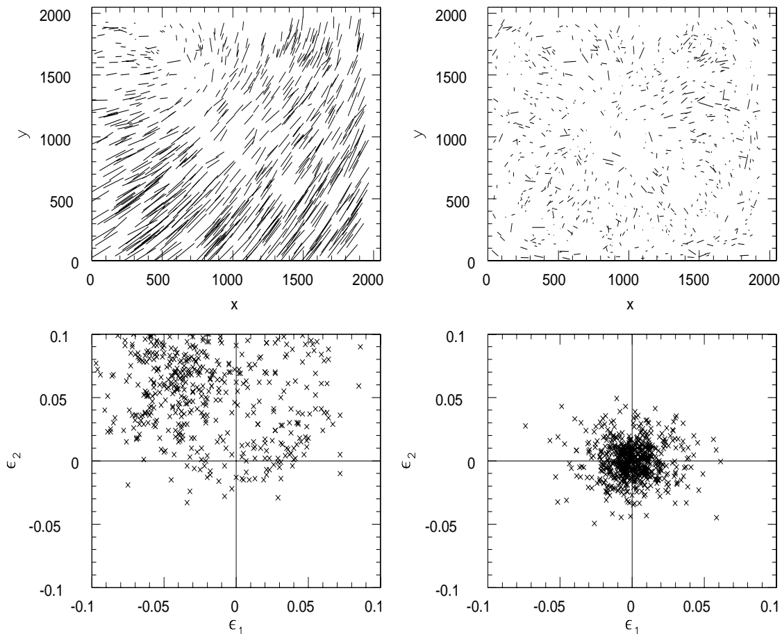
Fig. 10. A typical pattern of the PSF anisotropy (upper left) and components of the polarization vector (lower left) for an EMMI I -band frame (1 arcsec seeing). Also shown are the spatial distribution (upper right) and components of the polarization vector (lower right) after polynomial correction, as described in the text
