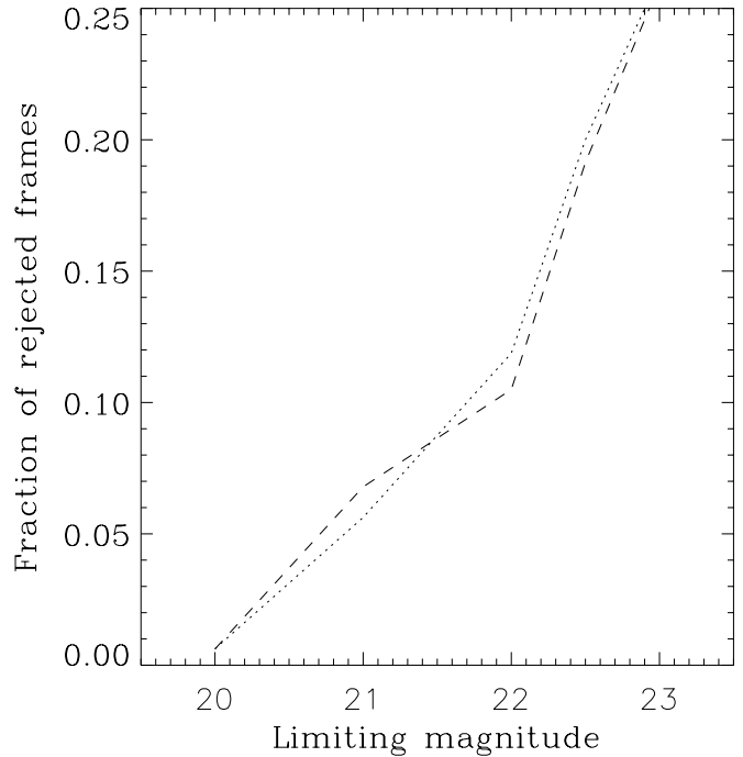
Fig. 30. Fraction of rejected tiles, corresponding to counts lower than 3\sigma from the mean in Fig. 29, as a function of the limiting magnitudes
