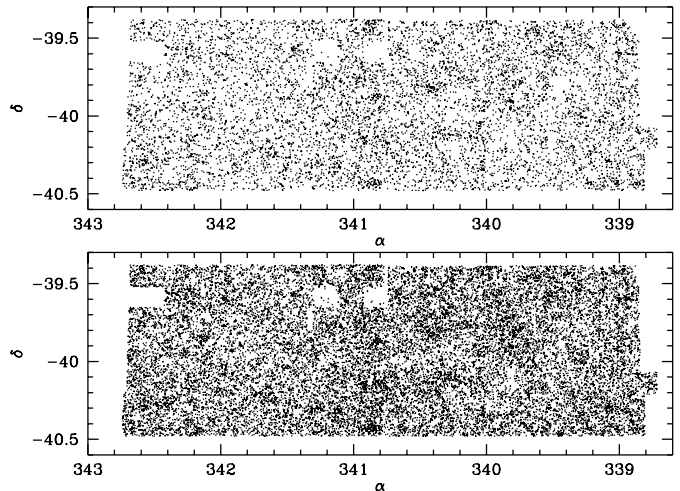
Fig. 16. Same as in previous figure showing the distribution of 9006 (upper panel) and 23129 (lower panel) galaxies for the same two limiting magnitudes as in Fig. 15. Again note the empty regions in the upper part of the patch caused by bad frames
