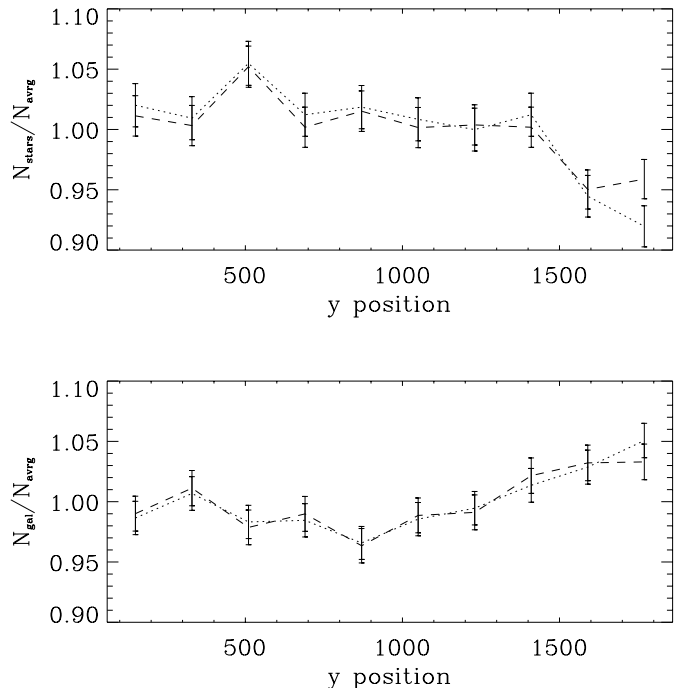
Fig. 18. As Fig. 17 but showing the detections in the north-south direction. Again at the “upper” edge of the chip we see a dip in the star counts and a corresponding increase in galaxy counts, which is due to the image distortions, see text for details
