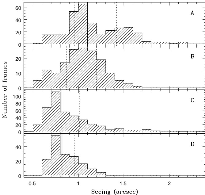
Fig. 3. Seeing distribution for all the EIS patches. The plot includes all the data taken in 1997. Note the great improvement of the seeing distribution, especially for patches C and D
