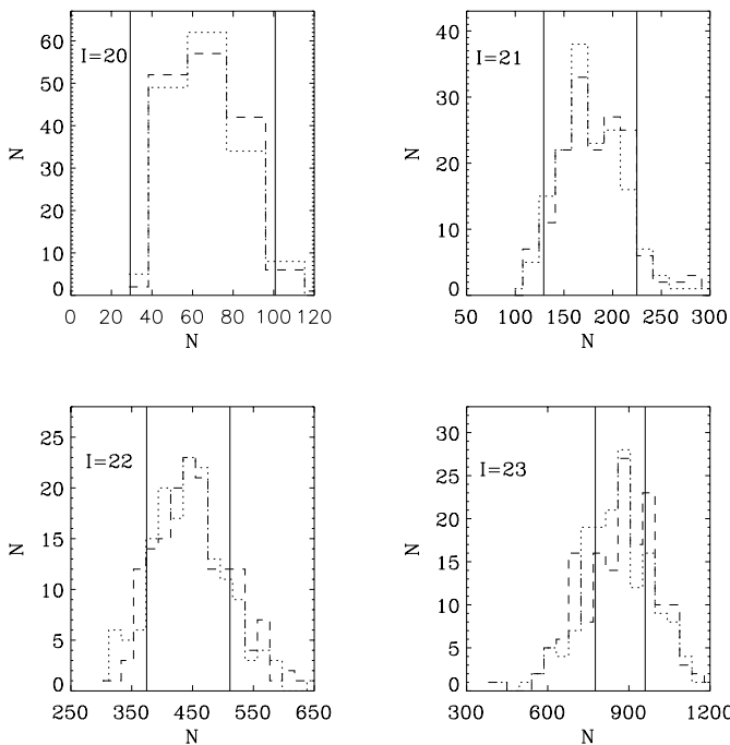
Fig. 29. Distribution of galaxy counts for the even (dotted line) and the odd (dashed line) catalogs as a function of limiting magnitude. The vertical lines correspond to the 3\sigma deviations from the mean, where \sigma includes the contribution from Poisson fluctuations and the galaxy clustering
