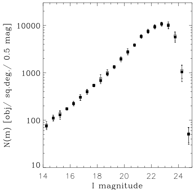
Fig. 23. The object counts as a function of magnitude as derived from the average of the counts in six odd (open squares) and even (filled squares) sub-catalogs. The error bars are the sample rms. In some cases the error bars are of the same size as the symbols
