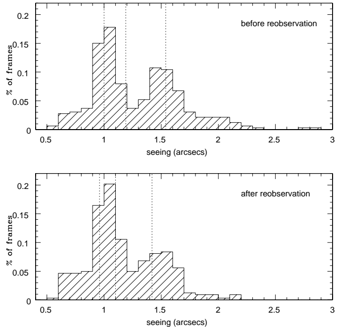
Fig. 2. Seeing distribution for patch A obtained from all observed frames (top panel) and only from the frames actually accepted for the survey (bottom panel). Vertical lines refer to 25, 50 and 75 percentiles of the distributions
