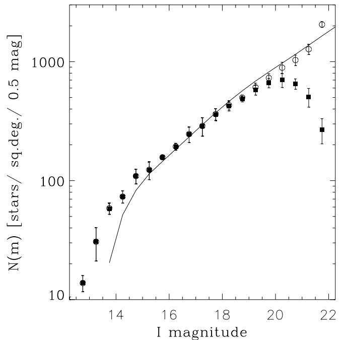
Fig. 25. The EIS star counts for stellerity index \geq 0.75 (filled squares) and for stellerity index \geq 0.5 (open circles) compared to the model by Mèndez & van Altena (1996) (solid line)
