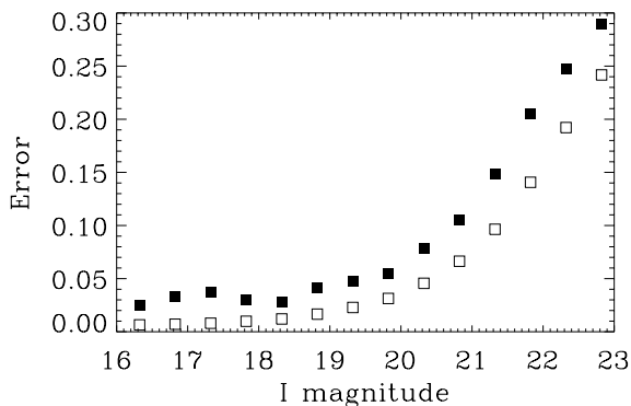
Fig. 22. Comparison between the standard deviation of the EIS-magnitude differences (filled squares) and the magnitude errors estimated by SExtractor (open squares) as function of magnitude
