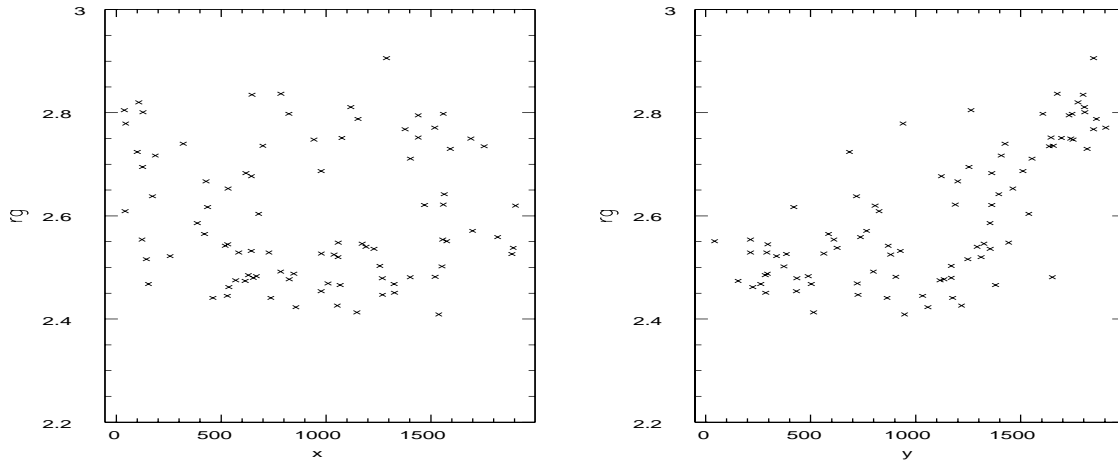
Fig. 11. Variation of the size of the PSF along the x -axis (left panel) and y -axis (right panel) of the CCD on EMMI. Note the increase in size near the top edge of the CCD. The quantity rg is the size of the stellar images as determined by the KSB algorithm. The image from which this result was derived has a seeing of \sim 1 arcsec
