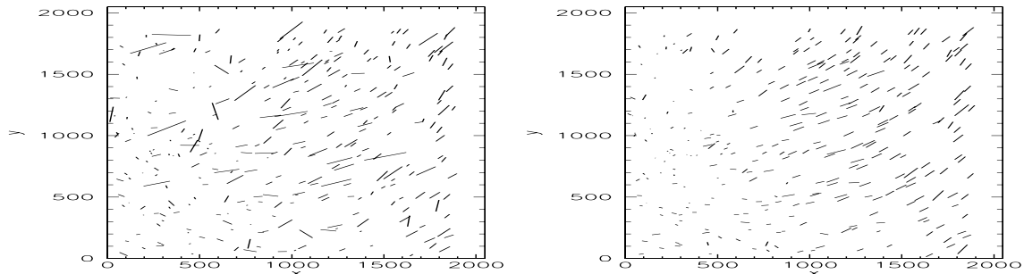
Fig. 9. Comparison of SExtractor and KSB shapes for stellar objects: The left panel shows the anisotropy structure as measured by SExtractor, while the right panel as measured by the KSB algorithm for the same stars
