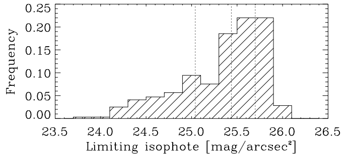
Fig. 6. Limiting isophote distribution for the patch A frames actually accepted for the survey. Vertical lines refer to 25, 50 and 75 percentiles of the distributions
