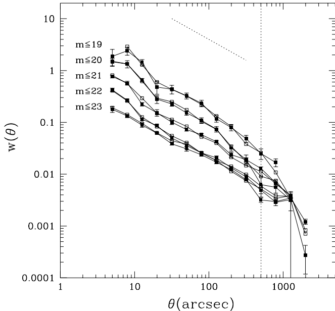
Fig. 26. Angular two-point correlation function calculated for the whole patch (even and odd catalogs) except the region defined by \alpha \gtrsim 340^\circ and \delta \gtrsim -39.8^\circ which has been removed for completeness problems. The dotted line represents a power-law with a slope of -0.8
