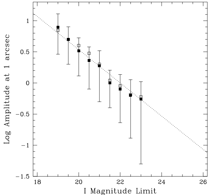
Fig. 27. Amplitude of the correlation function at 1 arcsec calculated from the best fits of Fig. 26 as a function of limiting magnitude. The dotted line is from Brainerd et al. (1996)
