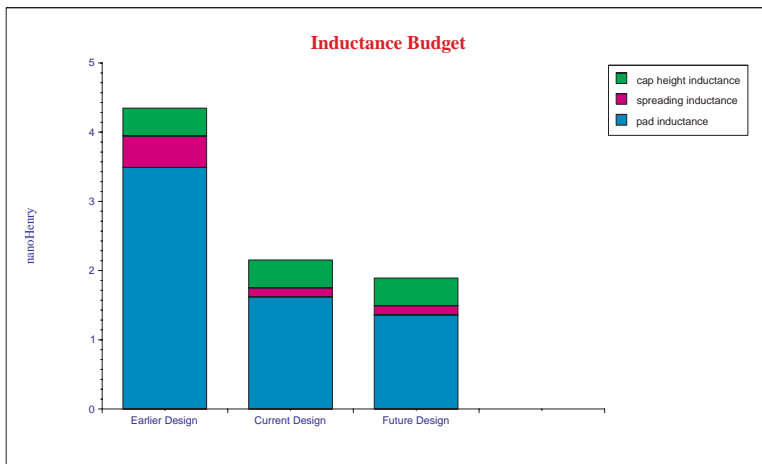
Figure 3. Total Inductance comparison.
