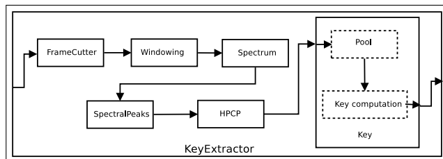
Figure 1. An example of the composite algorithm KeyExtractor combining the algorithms FrameCutter, Windowing, Spectrum, SpectralPeak, HPCP, and the Key algorithm composite itself.
