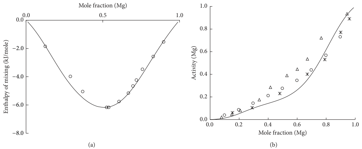
FIGURE 9: Calculated (a) enthalpy of mixing of liquid Mg-Ca at 1150 K: ○: [58]. (b) Activity of liquid Mg at 1100 K: △: [59] at 1200 K, *: [59] at 1080 K, ○: [60] at 1010 K.
