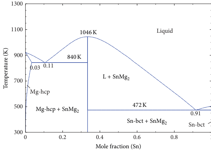
FIGURE 23: Mg-Sn phase diagram [22].
