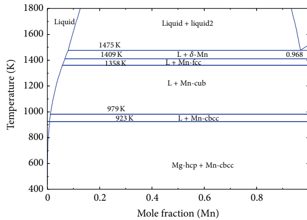
FIGURE 6: Mg-Mn phase diagram [32].
