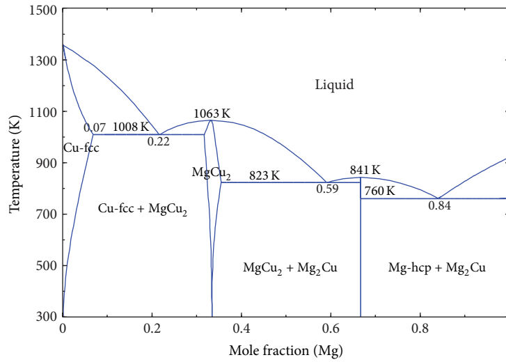
FIGURE 21: Mg-Cu phase diagram [66].
