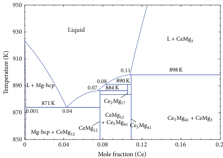
FIGURE 18: Magnified portion of the Mg-Ce phase diagram.
