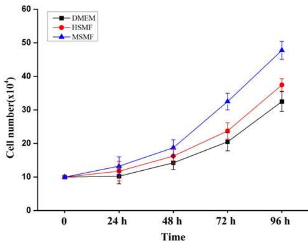
Figure 2. Growth curves for H9 cells cultured in KnockOut DMEM/F12 (DMEM), homemade serum-free medium (HSMF), and modified serum-free medium (MSFM).
