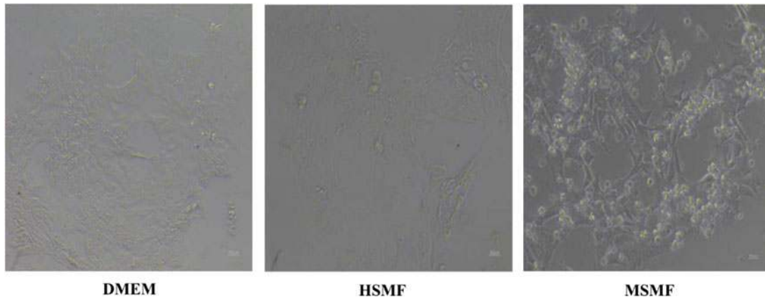
Figure 1. Cell morphology of H9 cells cultured under different conditions. DMEM, Dulbecco's modified Eagles's medium; HSMF, homemade serum-free medium; MSFM, modified serum-free medium.
