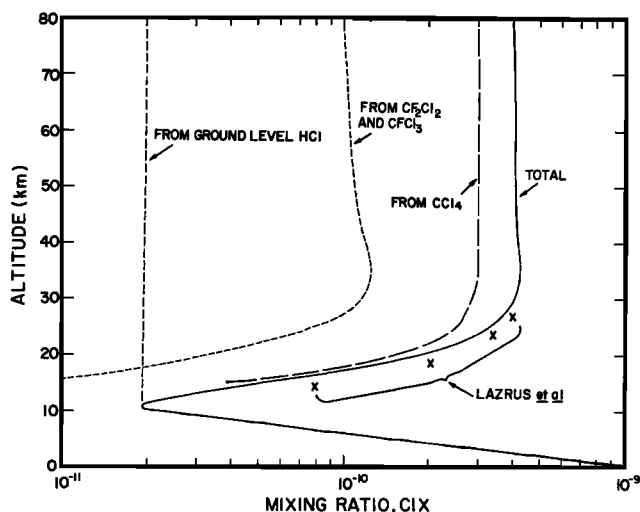
Figure 1. Computed ClX (HCl + ClO + Cl) mixing ratios versus altitude for late 1974. The ClX contribution from \text{CF}_2\text{Cl}_2 and \text{CFCl}_3 photolysis was calculated from the known history of anthropogenic emissions, that from \text{CCl}_4 as described in the text. Recent HCl measurements are shown by X's. Nearly all ClX is HCl below 25 km. A nominal tropospheric HCl profile is also shown, reflecting \text{H}_2\text{O} control.
