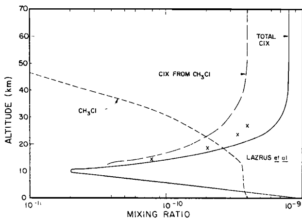
Figure 2. Computed ClX (HCl + ClO + Cl) mixing ratios versus altitude, due to a ground-level source of CH 3 Cl, and the computed CH 3 Cl profile for late 1974. The total ClX mixing ratio due to CF 2 Cl 2 , CFC1 3 , CCl 4 and CH 3 Cl is also shown, as are recent HCl measurements (X's) by Lazrus et al. [1974; 1975].
