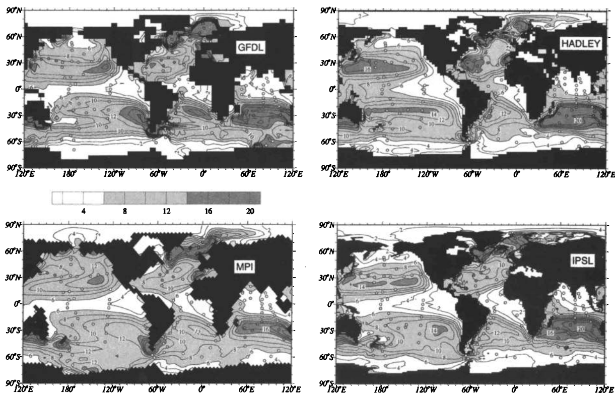
Figure 4. Bomb ^{14}\text{C} inventory (i.e., the vertical integral of the concentration) in units of 10^9 atoms ^{14}\text{C} \text{cm}^{-2} for the Princeton/GFDL, MPI, Hadley, and IPSL models. GEOSECS stations are marked with filled circles, shaded according to the data-based estimates of Broecker et al. [1995]. The same shading scheme is used for the data-based estimates (filled circles) and the model distributions (contour fields).
