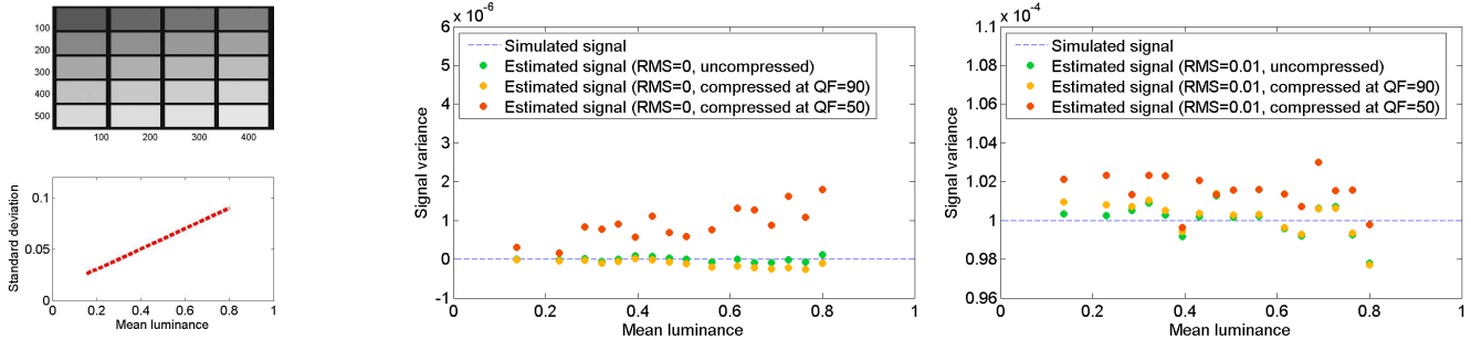
(a) Simulated video frame (top) and simulated NLF (bottom). (b) Mean (over space) estimated signal variance per mean (over time) luminance, from simulated videos containing no signal. (c) Mean (over space) estimated signal variance per mean (over time) luminance, from simulated videos containing a spatially invariant, temporally varying sine wave with RMS = 0.01 .
