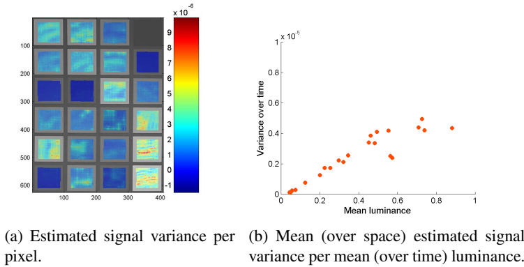
Figure 2: Estimated signal variance for a stationary color calibration target. The upper right region of the card was excluded from the visualization as it appeared to have extremely high noise levels that interfere with the visualization scale.
