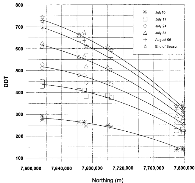
FIGURE 3. Relation between distance from Arctic Ocean (expressed as UTM northings, in meters) and thawing degree day sums (adjusted to sea level using a lapse rate of 0.64^\circ\text{C}/100\text{ m} ) at weekly intervals for the Flux study sites. Degree-day figures are totals for the period 23 June to 11 August. Coefficient of determination for second-degree polynomial regression equations is at least 0.98 in all cases.
