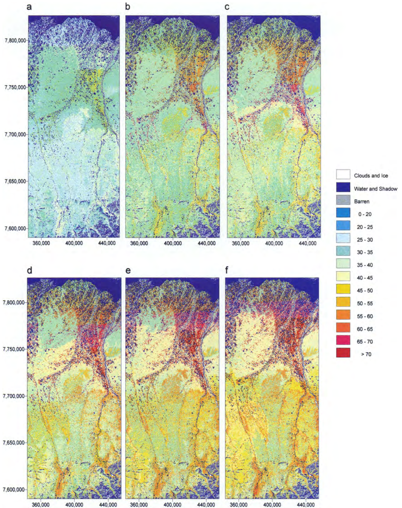
FIGURE 5. Active-layer thickness maps. These maps represent an integrated response to elevation-adjusted thawing degree-day totals, vegetation, moisture, and soils, through use of a regression equation for each land-cover type, and a topoclimatic index. (a) 10 July, (b) 17 July, (c) 24 July, (d) 31 July, (e) 06 August, (f) 11 August ("end of season"). Numbers along bottom and left margins are UTM coordinates (m), Zone 6. Legend given in cm.
