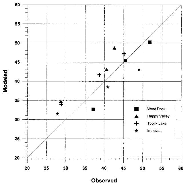
FIGURE 7. Results from accuracy assessment. Predicted mean values for the four 1 × 1 km ARCSS grids in and near the Kuparuk River basin are in close agreement ( \leq 6.1 cm) with those measured at the grids.
