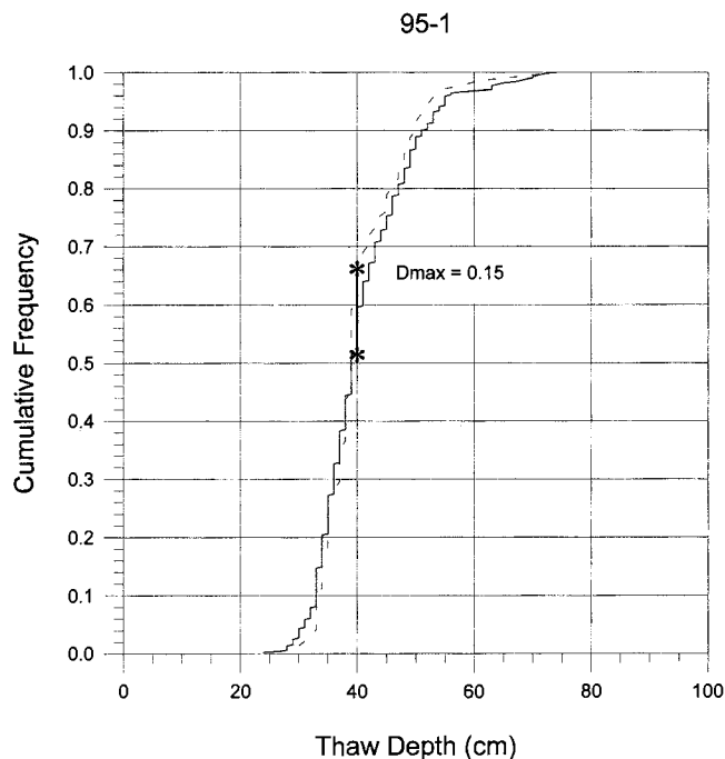
FIGURE 2. Comparison of results from 71-point sampling design (dashed line) with a more intensive 441-point probing effort (solid line) at the 95-1 Flux Study plot. D_{max} is the maximum difference, represented by stars, between the two cumulative frequency distributions, and forms the basis for the Kolmogorov-Smirnov goodness-of-fit test (e.g., Gibbons 1976: 56–75). No significant differences ( P = 0.1 ) were found between the sample and “population” distributions at any of the five plots examined using this strategy.
