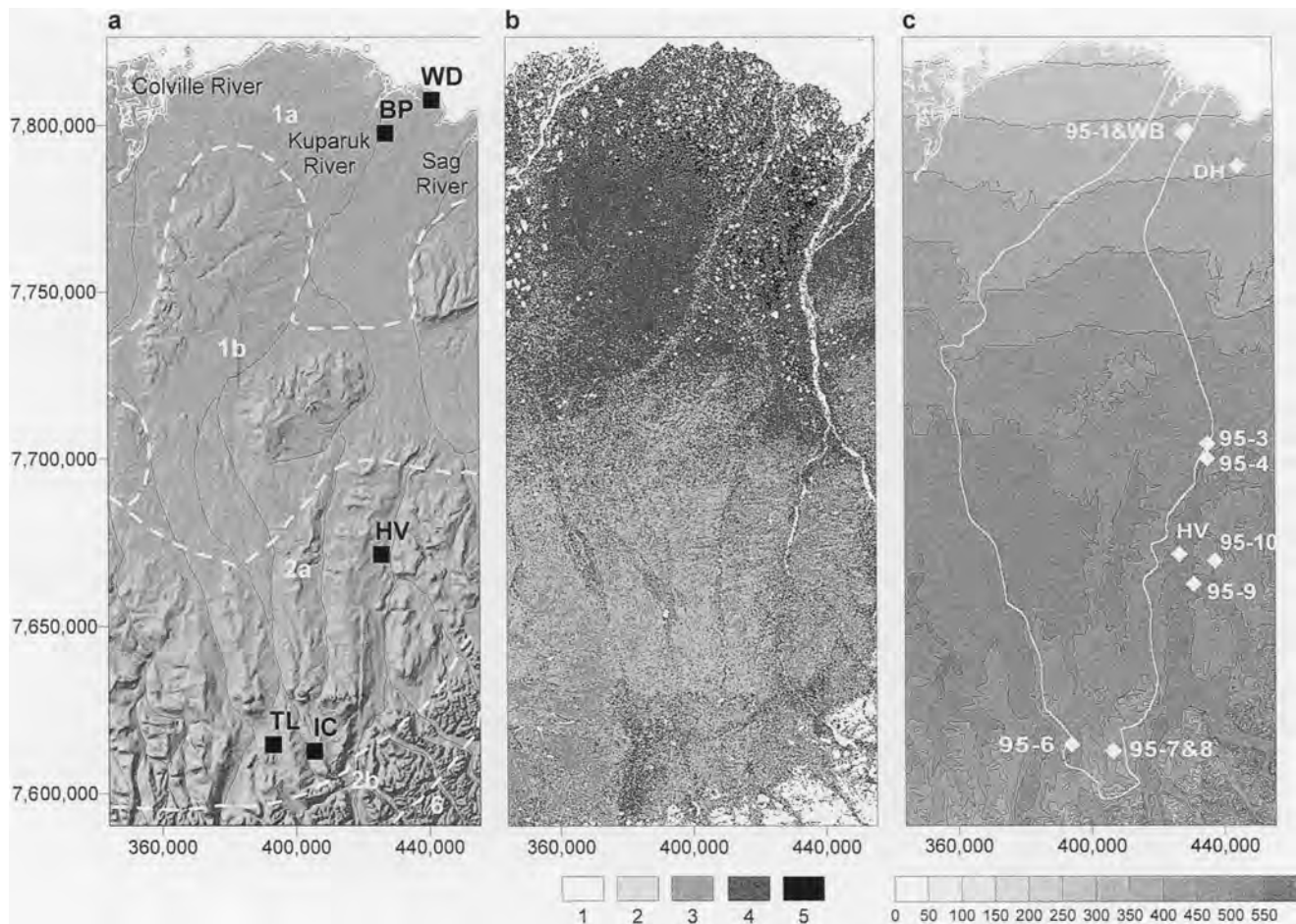
FIGURE 1. (a) Shaded relief map of study area, based on 787 \times 371 digital elevation model (300 m node spacing). Locations of ARCSS grids are shown by squares. BP = Betty Pingo; WD = West Dock; HV = Happy Valley; IC = Imnavait Creek; TL = Toolik Lake. Numbers along bottom and left margin are Universal Transverse Mercator (UTM) coordinates, Zone 6, expressed in meters. Generalized physiographic provinces (dashed white lines) are indicated, after Wahrhaftig (1965). 1: Arctic Coastal Plain Province: 1a: Teshekpuk Lake section; 1b: White Hills section. 2: Arctic Foothills Province: 2a: northern section; 2b: southern section. 6: Central and Eastern Brooks Range Province. (b) Land-cover map prepared from Landsat imagery (Auerbach et al., 1996). The version used in this study and shown here is a "thinned" version, in which only elements corresponding to positions of DEM nodes were employed. Land-cover categories denoted by numbers in legend are identified in Table 1. (c) Degree-day field for 11 August ("end-of-season"), obtained using the statistical relation of Figure 3 and environmental lapse rate to adjust values for nodes on the DEM. Labeled symbols indicate locations of Flux Study plots and sites where supplementary data were collected. Flux Study Plots (numbered sites) are described in Table 1. WB = Wet Betty Pingo, DH = Deadhorse, HV = Happy Valley. Kuparuk River basin is delimited by solid line.
