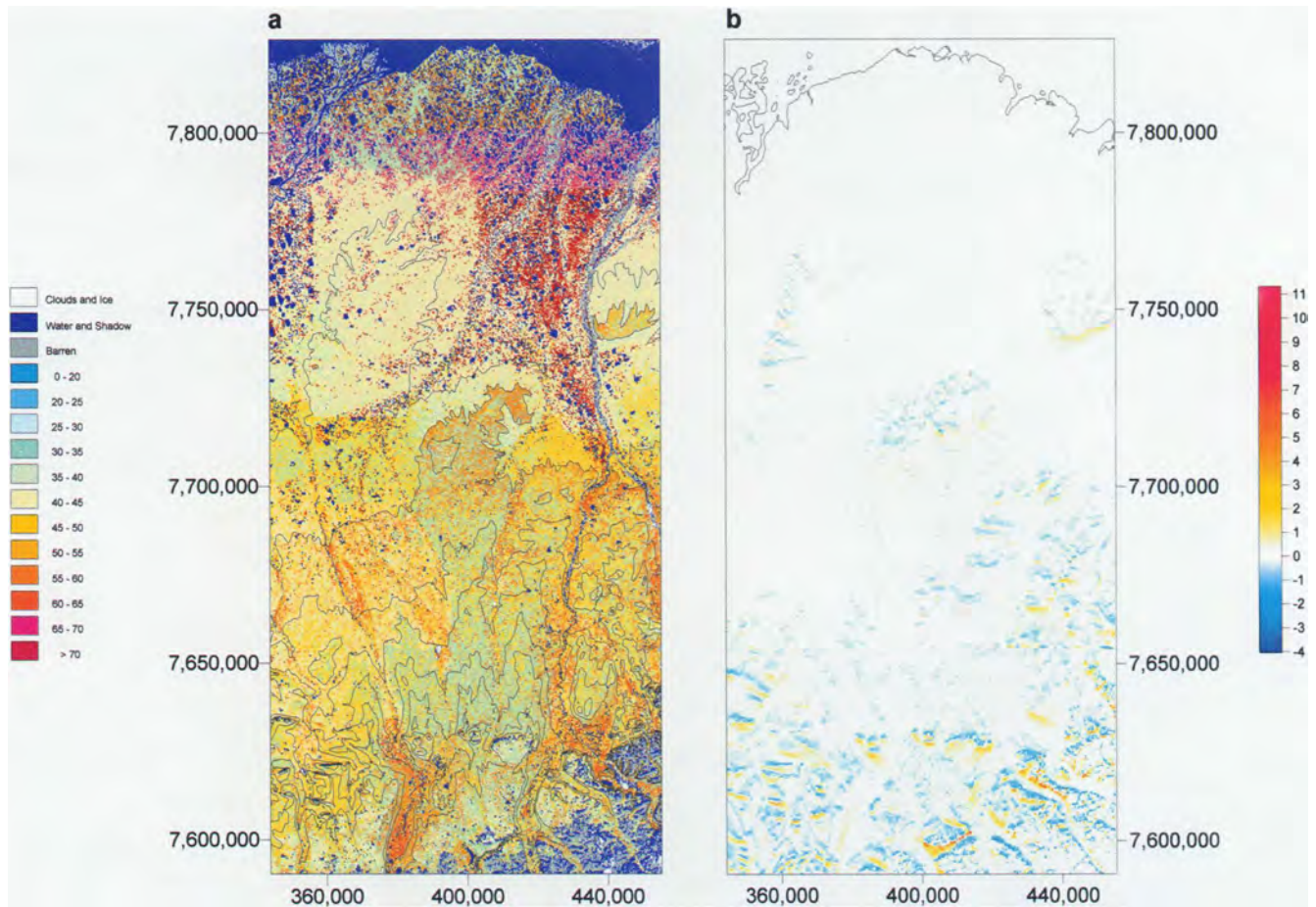
FIGURE 6. (a) Map for 11 August (Fig. 5f), showing relation between active-layer thickness and topography. Contour interval is 100 m, legend for active layer given in cm. Owing to complexity of terrain in Brooks Range (extreme southern part of study area), maximum contour shown is 800 m. (b) Difference map, depicting topoclimatic effects. Active layer is thinner (negative values; blue shading) on cooler, north-facing slopes and thicker on warmer, south facing slopes (positive values; yellow to red shading).
