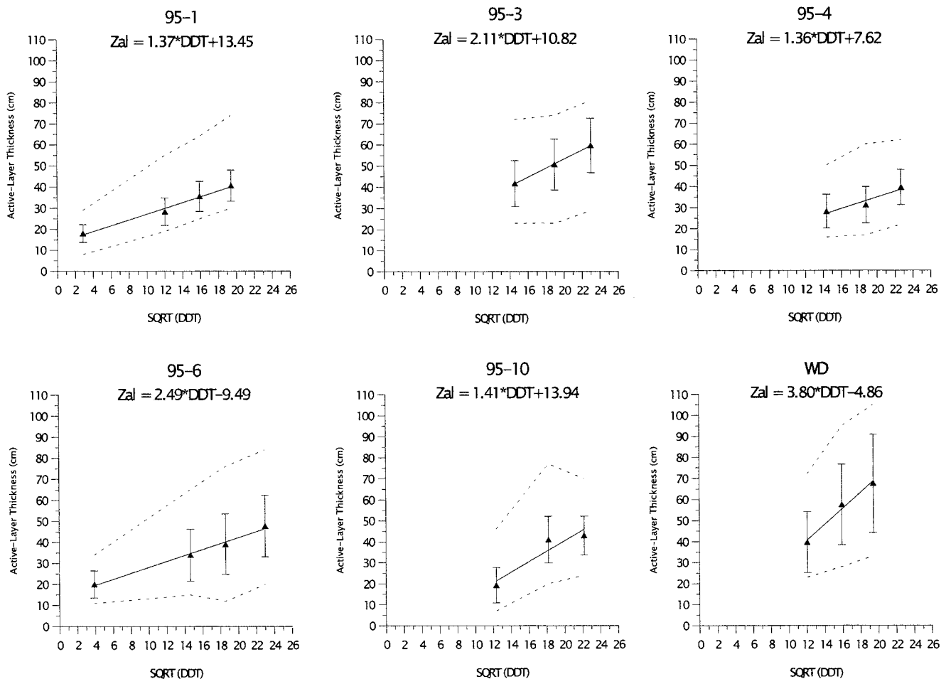
FIGURE 4. Statistical relation between mean thaw depth (71 replications per plot per date) and accumulated degree days (mast level) at individual Flux Study plots. Filled symbols represent mean thaw depth on specific probing dates, bars indicate standard deviations, and dashed lines show range (minimum and maximum) of values. Equations, represented by solid lines, represents the Stefan relation for each of the Flux Study plots, in the form given by equation (3).
