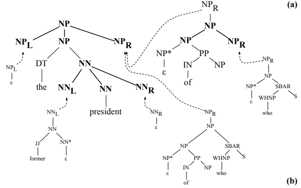
Figure 2: TIG-to-TSG transform: (a) and (b) illustrate transformed TSG derivations for two different TIG derivations of the same parse tree structure. The TIG nodes where we illustrate the transformation are in bold. (We suppress the rest of the transformational nodes.)
