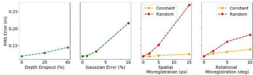
Fig. 10: Accuracy of D 3 Networks under Various Sparse Depth Errors. Under all potential error sources (with the exception of the unlikely random spatial mis-registration error), the D 3 network exhibits graceful error degradation. This error degradation is almost negligible for constant spatial mis-registration.
