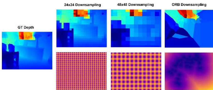
Fig. 2: Various Sparse Patterns. NN fill maps \mathcal{S}_1 (top row) and the sampling pattern Euclidean Distance transforms \mathcal{S}_2 (bottom row) are shown for both regular and irregular sparse patterns. Dark points in \mathcal{S}_2 correspond to the pixels where we have access to depth information.
