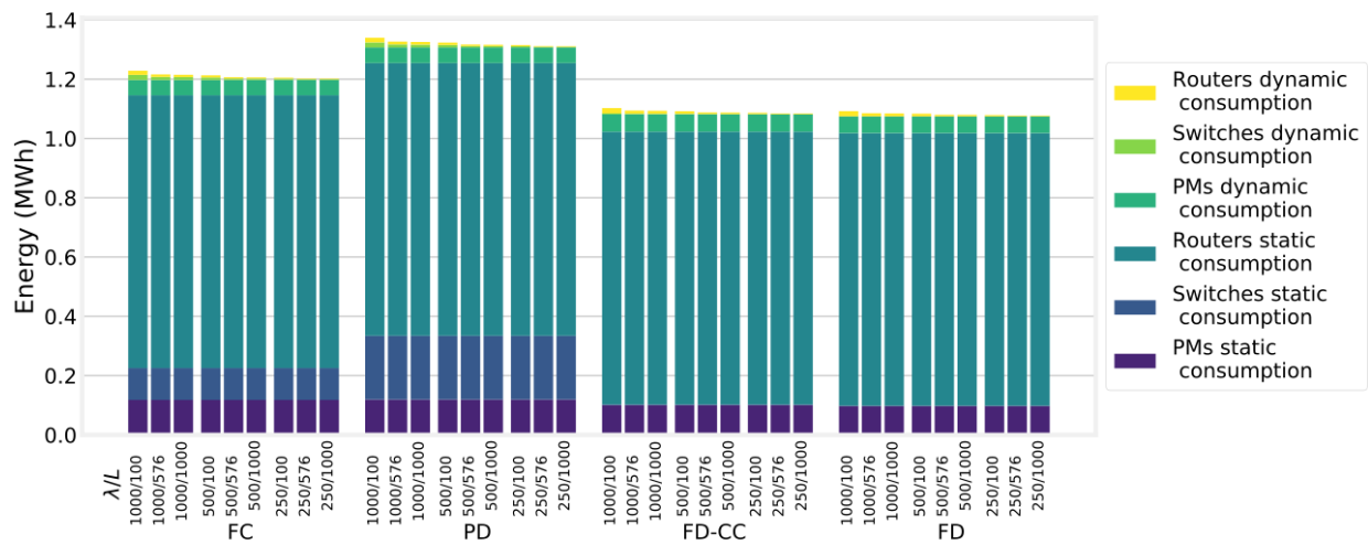
Fig. 8. Total energy consumption of different architectures for 1 hour
