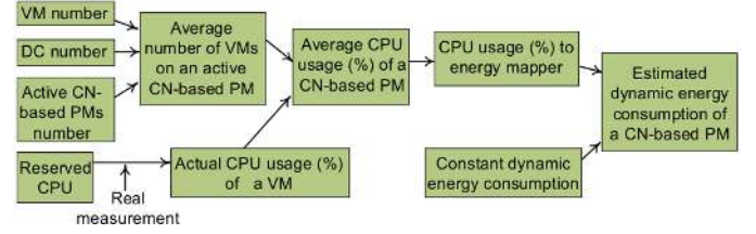
Fig. 5. Model for dynamic energy consumption of a CN-based PM
