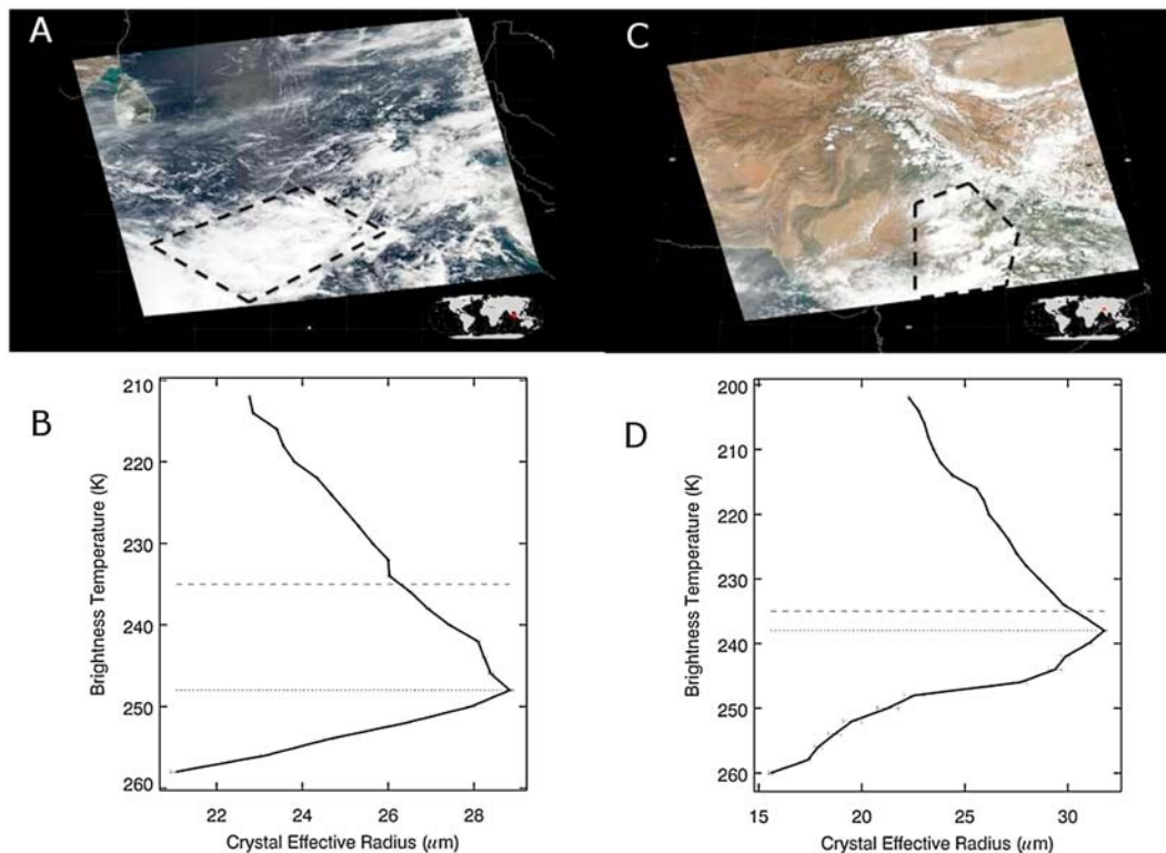
Figure 2. (a) Aqua MODIS true color image at 0815 UTC on 18 July, 2006. Analysis is done for the maritime cloud system (illustrated with black dashed lines). (b) The CER-BT profile for the DCC system selected in Figure 2a. The estimated glaciation temperature is about 248K (dotted line). The dashed line denotes the 235K (or -38^{\circ}\text{C} ) level. (c) Aqua MODIS true color image at 0730 UTC on 8 July, 2006. A deep convective cloud system located over the Indo-Gangetic Plain is encircled by dotted lines. (d) The CER-BT profile for the DCC system selected in Figure 2c.
