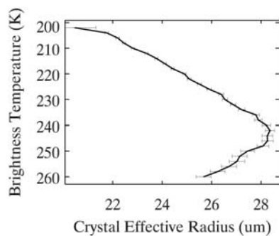
Figure 3. Smoke affected areas over Amazon show elevated glaciation height (or lower temperature). The glaciation temperature inferred from this ensemble profile is around 242K.
