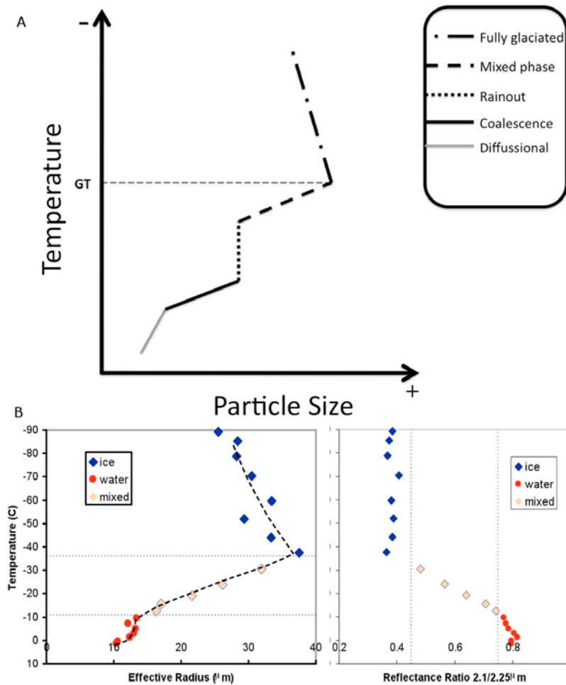
Figure 1. (a) A conceptual diagram of cloud particle size vertical evolution inside a DCC. It is a slightly modified picture from Rosenfeld and Woodley [2003] based on results of Yuan and Li [2010]. (b) Cloud side scanner retrievals of (left) particle size and (right) cloud phase. Independent reference can be made about the glaciation level from either one of these plots using indirect (Figure 2b, left) and direct arguments. This validates main arguments used in this paper. Figure is extracted from Martins et al. [2007].
