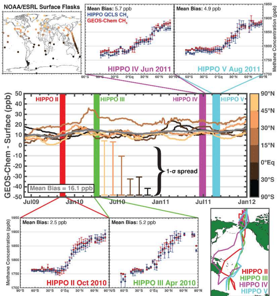
Figure A3. Global evaluation of the GEOS-Chem methane simulation at 4^{\circ} \times 5^{\circ} resolution (using prior emissions) with observations from the NOAA/ESRL surface flask network (top left panel colored by latitude) and HIPPO aircraft deployments. The central panel shows 3-month running medians for 2009–2011 of the difference between GEOS-Chem and the flask data in different latitudinal bands. The gray line is for all of the observations. Error bars for the running medians are offset from the lines for clarity. Latitudinal profiles across the Pacific for the four HIPPO deployments over the period are also shown: in those panels the symbols represent the pressure-weighted tropospheric average concentrations and the vertical bars are the standard deviation. Stratospheric air is excluded based on an ozone–CO concentration ratio larger than 1.25 (Hudman et al., 2007). Bottom right panel shows the HIPPO flight tracks.
