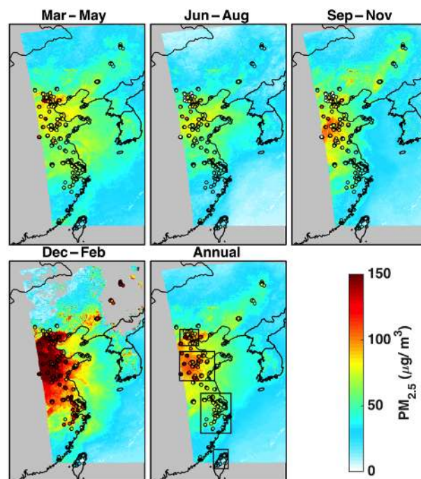
Figure 3. Seasonal and annual distribution of PM 2.5 concentrations at 6 km by 6 km resolution over East Asia for 2013. The background color indicates averages of GOCI-derived daily surface PM 2.5 concentrations. Filled circles represent averages of daily ground-based measurements of PM 2.5 . Gray denotes missing values. Boxes in the annual map denote regions used for monthly comparisons in Fig. 5 from top to bottom: Beijing and surrounding areas, Shandong and surrounding regions, Shanghai and surrounding areas and northern Taiwan.
