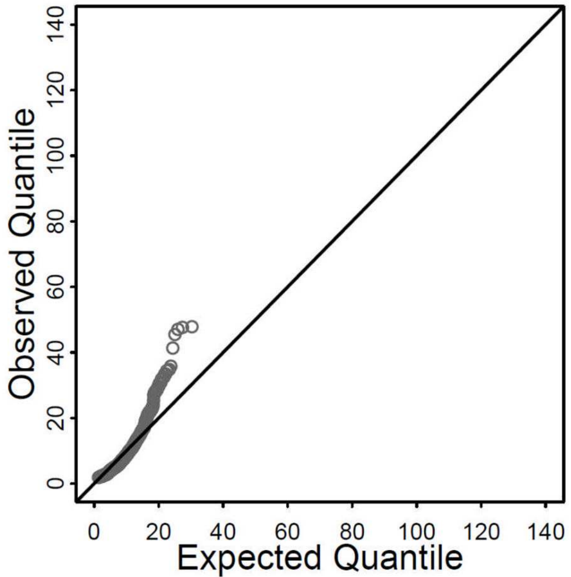
Figure 2. Multivariate QQ Plot of Observed Exogenous Variables (Excluding Product Indicators) of the Illustrative Example
