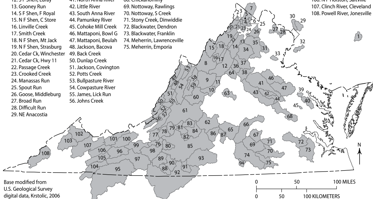
Figure 3: Names and locations of watersheds referenced in this study.
