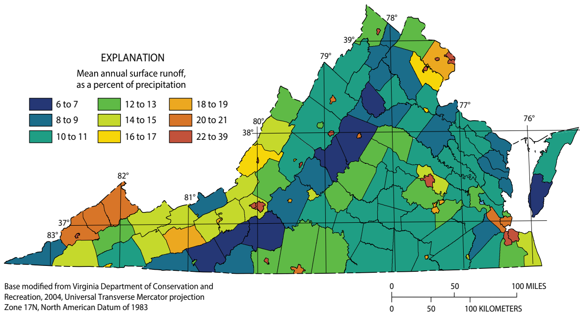
Figure 14: Estimates of surface runoff as a percent of precipitation in Virginia from 1971-2000 by locality.
