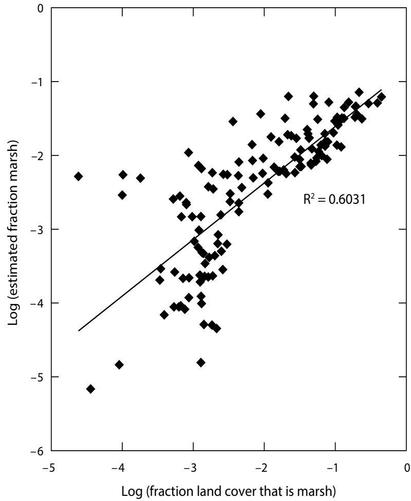
Figure 11: Comparison of fraction of locality land cover that is marsh and that estimated using temperature and topographic slope.
