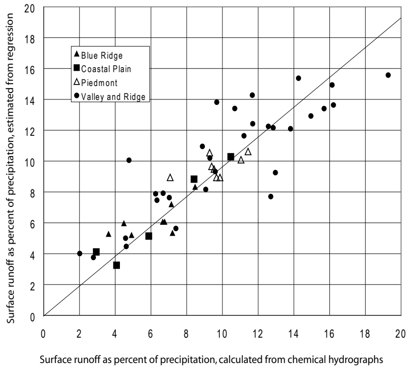
Figure 13: Comparison of calculated surface runoff versus that estimated by the regression.
